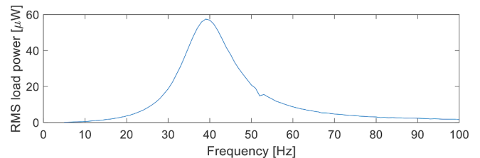
Fig. 14. Frequency response using parameterization tuned to 40 Hz.
