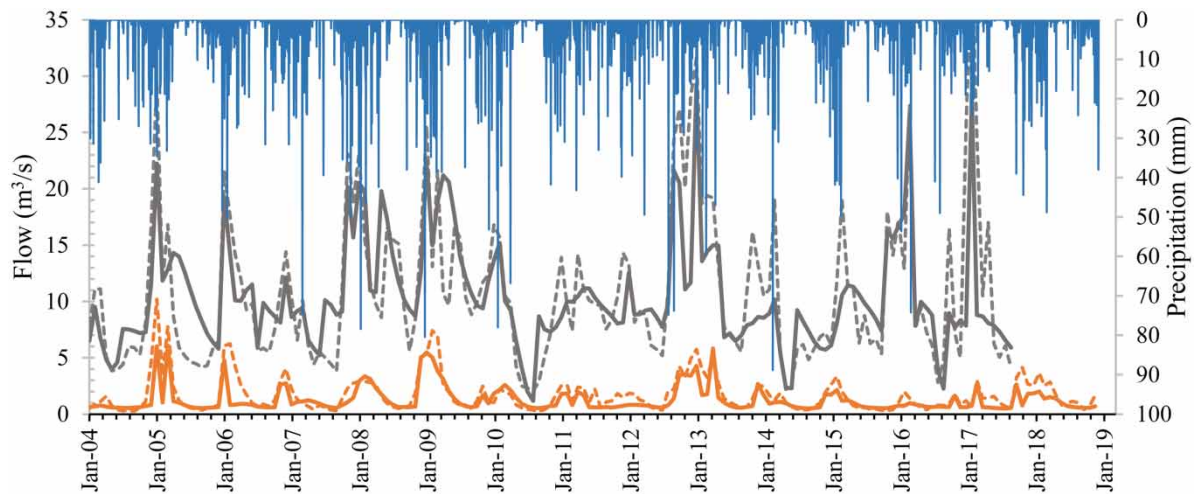
Figure 2 | Graphical comparison of simulated streamflow against observed flow for subbasins 1 and 10 calibration (January 2004–December 2011) and validation (January 2012–December 2018) periods. Subbasin 1 is depicted in grey and subbasin 10 in orange. Continuous and dashed lines represent simulated and observed data, respectively. The blue line in the secondary vertical axis shows the daily precipitation. Please refer to the online version of this paper to see this figure in colour: https://doi.org/10.2166/wh.2022.266 .
