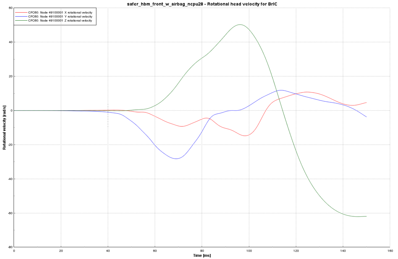
Fig. A2. Head rotational velocities in the FF load case with NCPU=28 on the VC system, filtered with a Channel Filter Class (CFC) 60 filter.
