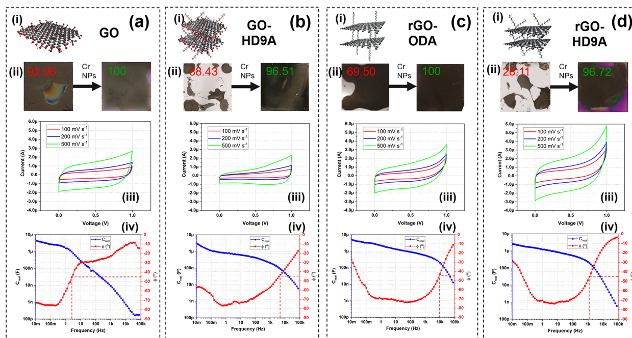
Figure 3. (i) Schematic representation of the atomic configuration. (ii) Improvement in coverage of spin-coated electrodes after addition of a Cr nanoparticle layer (experiments conducted on a 1 cm 2 Si chips). (iii) cyclic voltammograms of MSC with 20 fingers with 40 μm spacing fabricated by process described in 1 at different scan rates ranging from 100–500 mV s -1 . (iv) Bode plot for fabricated MSCs, for 3 g/L (a) GO in H 2 O (reduced postprocess), (b) GO-HD9A in ODCB (reduced postprocess), (c) rGO-ODA in ODCB, and (d) rGO-HD9A in ODCB.
