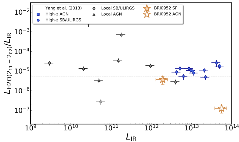
Figure 6.5: L_{\text{H}_2\text{O}}/L_{\text{IR}} versus L_{\text{IR}} for BRI0952 and a sample of other local and high-redshift galaxies. Two stars are shown for BRI0952, the empty star designates the L_{\text{IR,AGN}} while the filled star shows the L_{\text{IR,SF}} . The ratio for BRI0952 is similar to other high-redshift AGN and starburst galaxies when using the L_{\text{IR,SF}} . Figure from Kade et al. (in prep).
