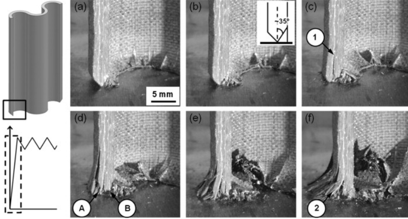
Figure 1.1: Laminated fibre composite subjected to crushing. Failure mechanisms: bending of plies (A), compressive failure (B), delamination in mode I (1), and delamination in mixed mode (2). From Grauers (2013) [3]. Reprinted with permission.
