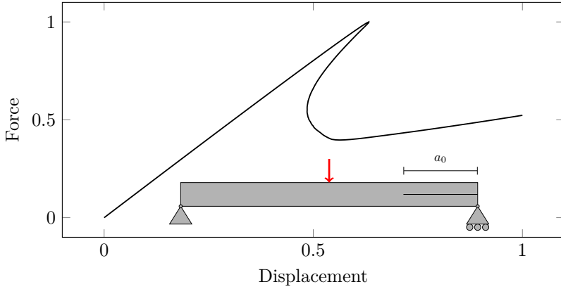
Figure 3.1: Illustration of snap-back behaviour when simulating an end-notch-flexure test (simply supported beam with an initial crack and applied load in the centre).
