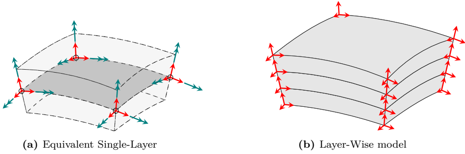
Figure 1.2: Illustration of two modelling approaches for fibre composites. Red arrows symbolise displacement degrees of freedom and green arrows symbolise rotational degrees of freedom.
