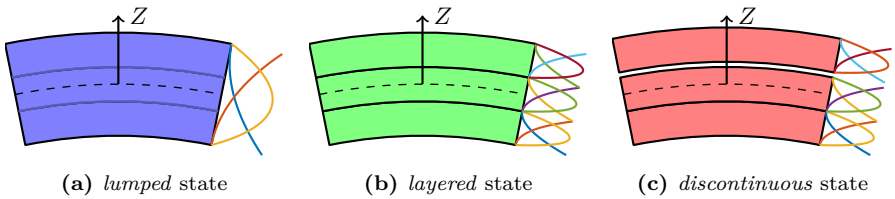
Figure 2.6: The three configurations considered in this work, denoted lumped , layered and discontinuous . The knot vectors, \Xi , are, a) [-1, -1, -1, +1, +1, +1] b) [-1, -1, -1, -\frac{1}{3}, -\frac{1}{3}, +\frac{1}{3}, +\frac{1}{3}, +1, +1, +1] and c) [-1, -1, -1, -\frac{1}{3}, -\frac{1}{3}, +\frac{1}{3}, +\frac{1}{3}, +\frac{1}{3}, +1, +1, +1] .
