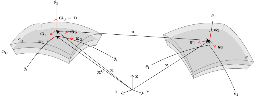
Figure 2.5: Kinematics of the continuum shell in the undeformed and deformed configuration.
