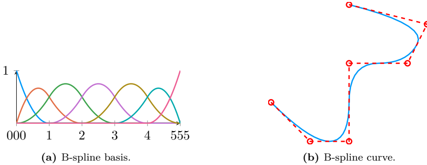
Figure 2.2: Illustration of B-Spline basis functions and a B-spline curve. The control points in (b) are illustrated as red circles.
