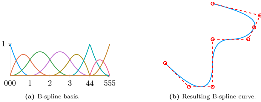
Figure 2.4: The basis functions and resulting B-spline curve after a knot has been inserted at \xi = 4 .
