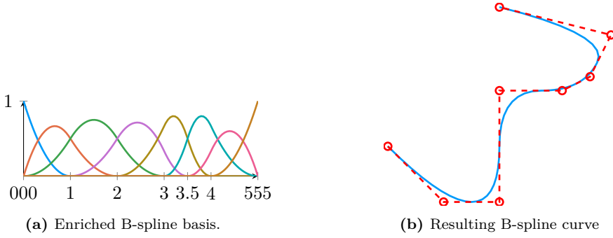
Figure 2.3: The basis functions and resulting B-spline curve after a knot has been inserted at \xi = 3.5 .
