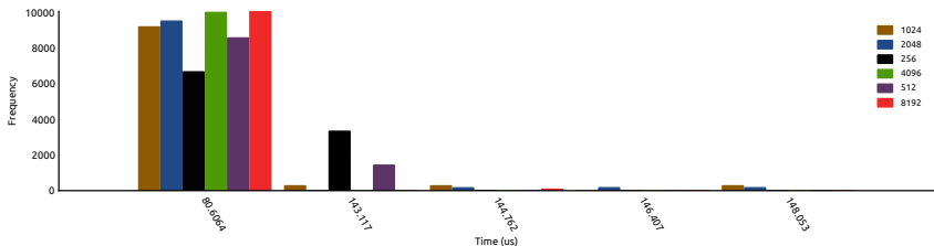
Figure 9 Response time measurements at different sizes of the heap to identify effects of garbage collection. This data is collected on the NRF52 microcontroller running SynchronVM on top of the Zephyr OS. Each bucket size is approx 1.65us. Uses 10000 samples.
