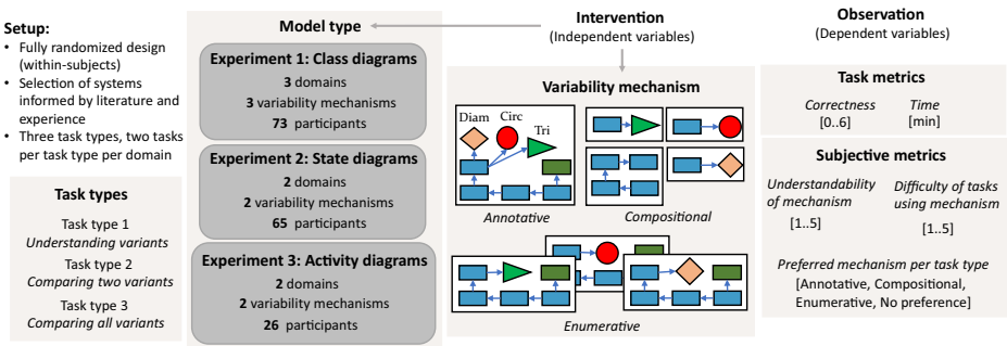
Fig. 4 Methodology overview
