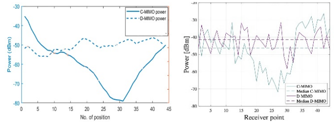
(a) Measurements, from [5] (b) Simulations Fig. 5. Comparison of received power at each of the 44 user positions, using a) testbed measurements and b) radio propagation simulations.
