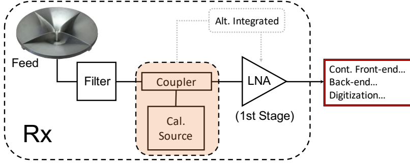
Figure 2.3: Typical wideband receiver chain illustrated including the alternative option to include gain calibration directly in the LNA [13], [25].
