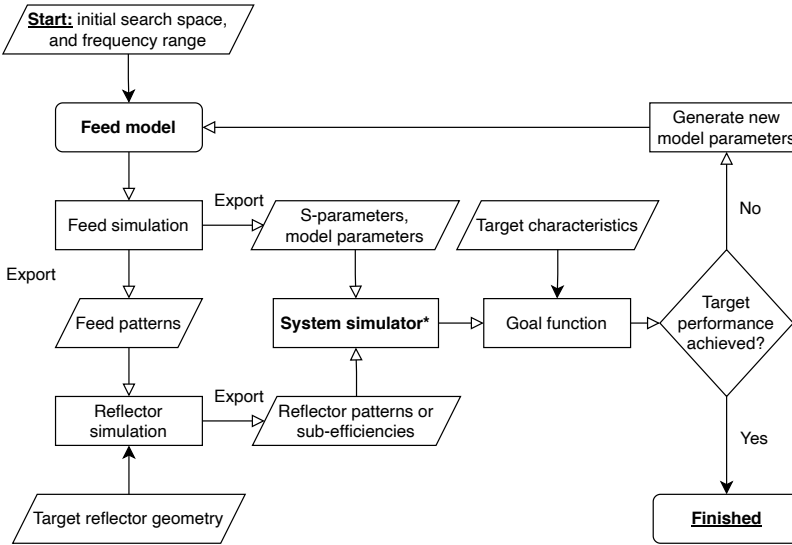
Figure 3.9: Typical optimization scheme in wideband feed design. *System simulator can be different depending on the application, and can also include parts of the outlined schematic.
