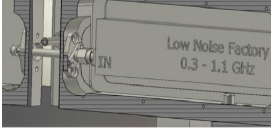
Figure 3.21: Integration of LNA directly inside QRFH ridge [26].
