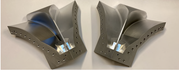
Figure 3.15: Horn and ridge machined as one part in quarter sections
