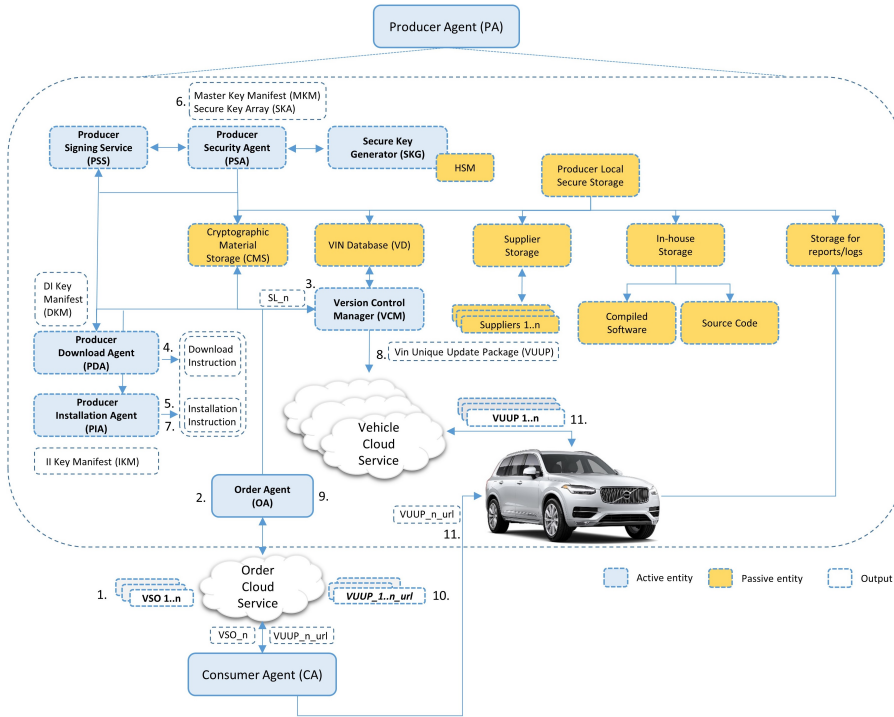
Figure 5.1: Data distribution in the backend
