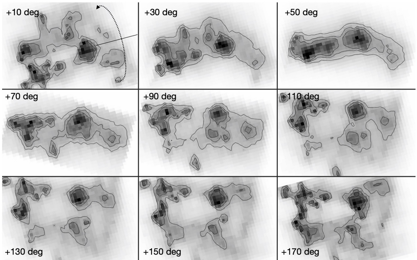
Fig. A.5. Chamaleon cloud complex viewed from various viewing angles rotating with respect to the y axis. The number in the panels indicates the rotation from the POS angle. The rotation direction is indicated in the top-left panel. The contours show the levels of A_G = \{0.5, 0.75, 1\} mag.
