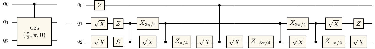
FIG. 8. Decomposition of the CCZS(\pi/2, \pi, 0) gate into single-qubit and CZ gates, obtained using Qiskit [154]. For the single-qubit gates, we use the notation S = \sqrt{Z} = Z_{\pi/2} and \sqrt{X} = X_{\pi/2} . Note that this decomposition requires qubit 2 being placed in the middle of the linear chain, since it has to perform CZ gates with both qubit 0 and qubit 1.
