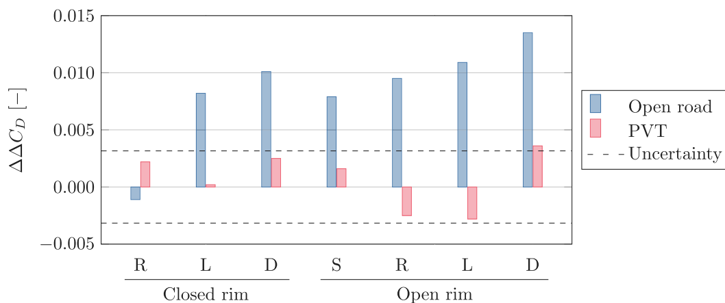
Fig. 26. \Delta\Delta C_D showing the difference between open road (CFD open road and corrected experimental data) and PVT (CFD PVT and uncorrected experimental data) conditions. The baseline configuration is the slick tyre with closed rim.
