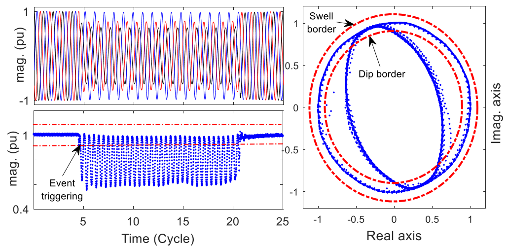
Figure 2. The waveform (upper left), the modulus of the SPM as a function of time (lower left), and the corresponding SPM (right) of a typical voltage dip. The dashed lines and circles show the dip/swell detection border (thresholds).
