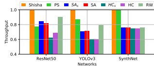
Fig. 5: Throughput of search schemes normalized to ES
