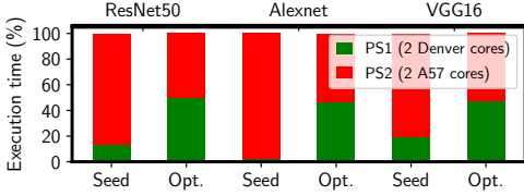
Figure 4: Percentage execution time of CNN pipelines with seeds and optimal configurations
