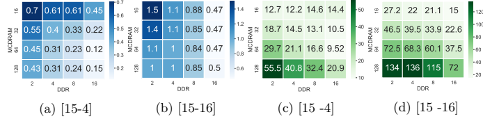
Fig. 2: (a) & (b) Execution time [s], (c) & (d) Parallel cost ( Core\ count \times execution\ time ) of STREAM Triad with data distribution [X-Y], where X = GBs placed in MCDRAM and Y = GBs placed in DDR
