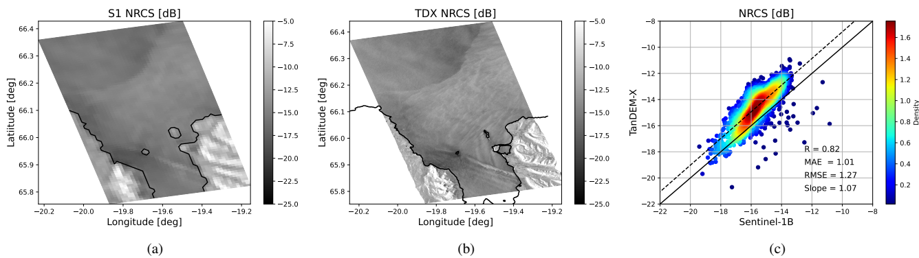
Fig. 5. Comparison of the NRCS (in dB) measured by Sentinel-1 and TanDEM-X over the Iceland Sea on 2020-06-26 18.00. (a) Sentinel-1 NRCS, (b) TanDEM-X NRCS, (c) scatter plot. R: correlation coefficient, MAE: mean absolute error, RMSE: root mean squared error.
