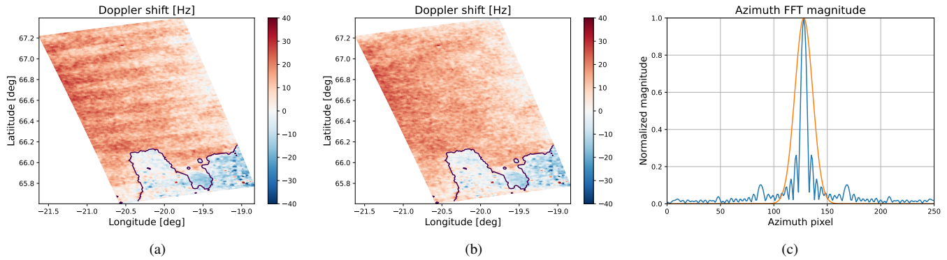
Fig. 3. Removal of the scalloping effect, Sentinel-1A, 2020-06-26, Iceland Sea. (a) before desclopping, (b) after desclopping, (c) a cut through the center along the azimuth direction of the power spectrum (blue curve) and the Gaussian window (red curve) used to filter the scalloping signal. The spectrum is zero padded by a factor four to improve the visibility.
