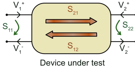
Figure 2.4: Illustration of the scattering parameters of a two-port network.
