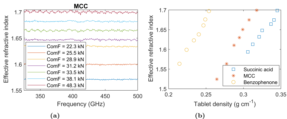
Figure 5.1: a) Effective refractive index versus frequency for MCC, for different compaction forces. Higher compaction force increases the effective permittivity. b) Effective refractive index versus tablet density, for Benzophenone, MCC, and Succinic acid. For a specific effective refractive index, the Benzophenone tablets show the lowest tablet density, followed by MCC and Succinic acid tablets, respectively.
