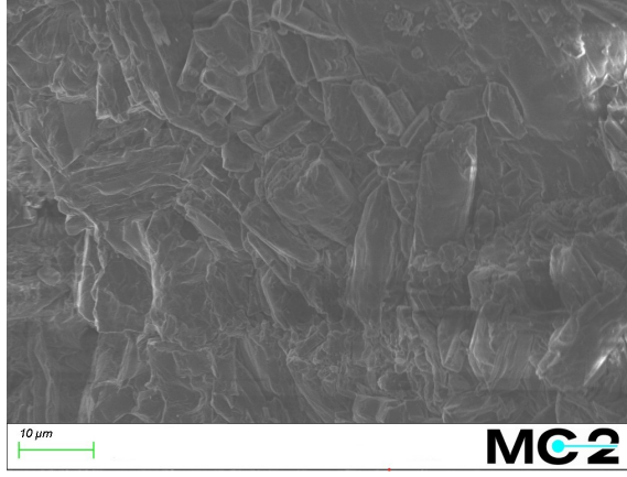
Figure 5.5: Scanning electron microscopy of cross-section of tablet (experiment number 3 in table 3.4). The fragmentation of particles while tableting process is clearly seen in this picture.
