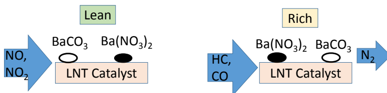
Figure 2.8: Simplified mechanism of lean \text{NO}_x trap shown during \text{NO}_x adsorption under fuel lean conditions (left) and \text{NO}_x reduction under fuel rich conditions (right).
