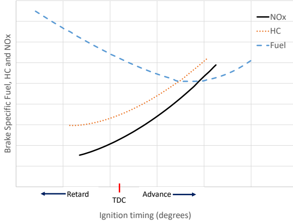
Figure 2.16: Effect of ignition timing on fuel consumption and engine emissions of HC and NOx.
