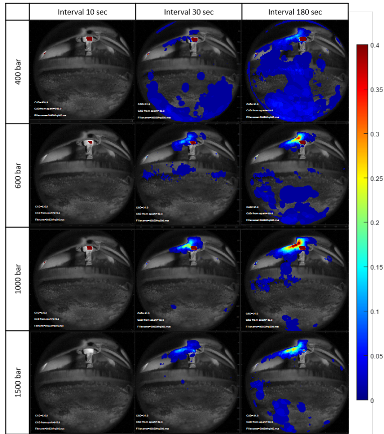
Figure 5.18: Relative frequencies of observation for luminous flames during the first 10 cycles after motoring for various motoring durations and injection pressures under simplified transient conditions
