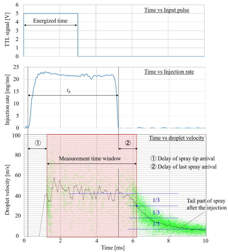
Figure 3.10: Measurement time window for PDI experiments.
