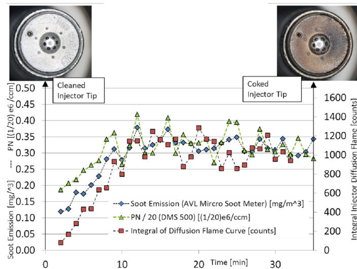
Figure 2.14: An example of PN drift caused by injector tip deposition [4]
