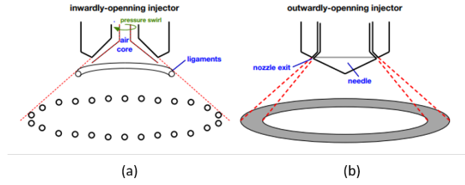
Figure 2.3: Schematic depictions of hollow-cone sprays and film structures. (a) Swirl nozzle. (b) Outward-opening nozzle [56].
