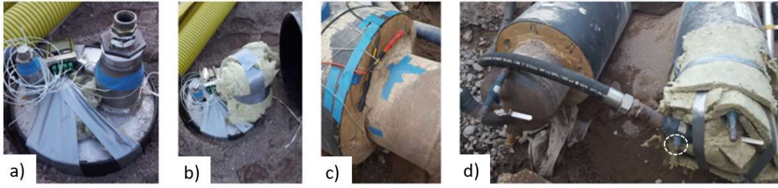
Fig. 11. a) TC attached to the drainage valve, to the right; b) the same valve after insulation with mineral wool. c) The service pipe at the excavation with TCs measuring T_s and crocodile clamps on the ends of the copper wires, connected to a multimeter; d) the same pipe, to the right, after insulation with mineral wool. White dotted circle shows the valve on the flexible pipe, which was switched off for the shutdown.
