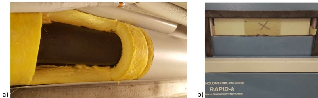
Fig. 9. a) The pipe after removing a piece of insulation. b) Part of the removed piece of insulation (x) when tested in the GHFM.
