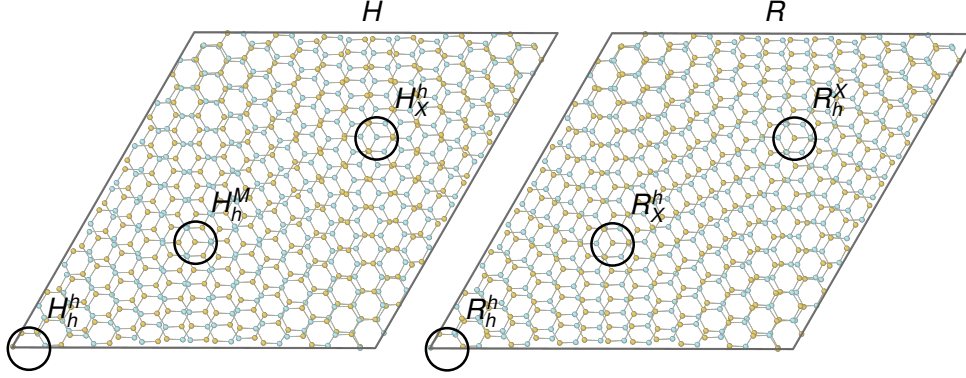
Figure 2.8: H and R stacked moiré superlattices at a twist angle of 4.41^\circ with the high-symmetry positions indicated. The atomic structures were visualized using the software OVITO [57].
