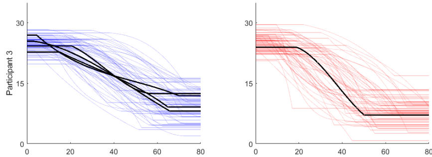
Figure 23. Posterior predictive checks for baseline (light blue, left) and cyclist (light red, right) conditions, plotted against the raw data from the experiment (solid black curves)
