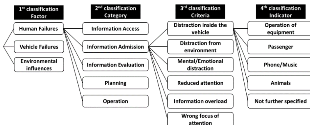
Figure 6. Example of ACAS classification in GIDAS, adapted from Schindler et al. (2022)
