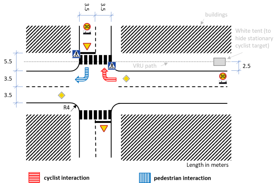
Figure 11. Intersection layout for the experiment at the AstaZero test track (the arrows show the places of the interactions seen in Figure 9), adapted from Schindler and Bianchi Piccinini (2021)
