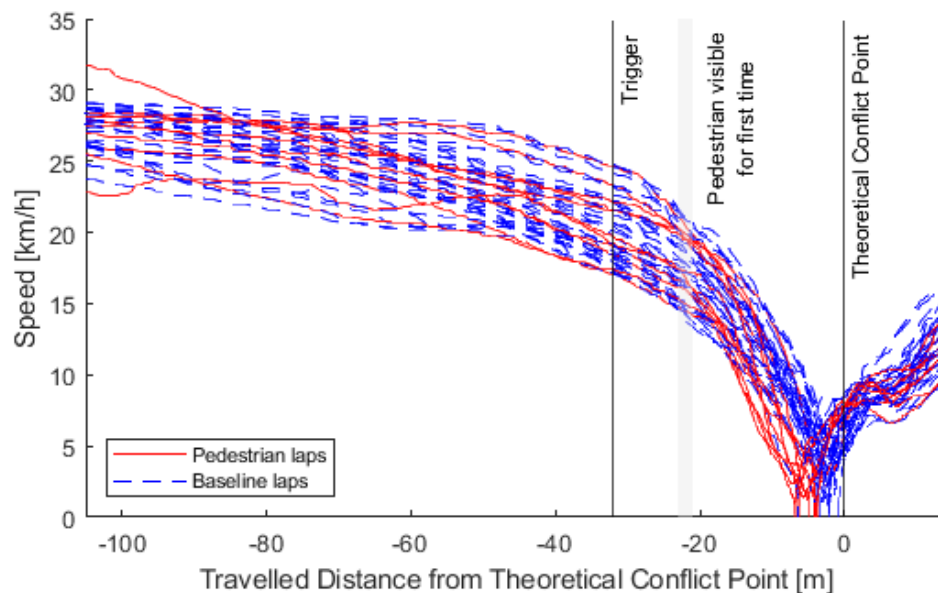
Figure 17. Speed over distance travelled for pedestrian encounters, adapted from Schindler and Bianchi Piccinini (2021)
