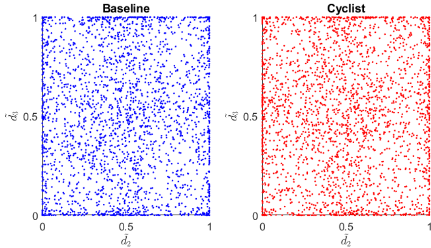
Figure 22. Prior predictive draws of \tilde{d}_2 and \tilde{d}_3 in beta space, from Schindler et al. (2021)
