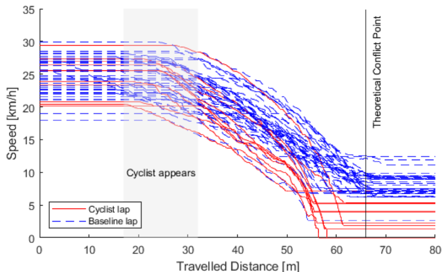
Figure 20. Fitted speed over distance travelled for first right turn manoeuvre (cyclist encounters), adapted from Schindler et al. (2021)
