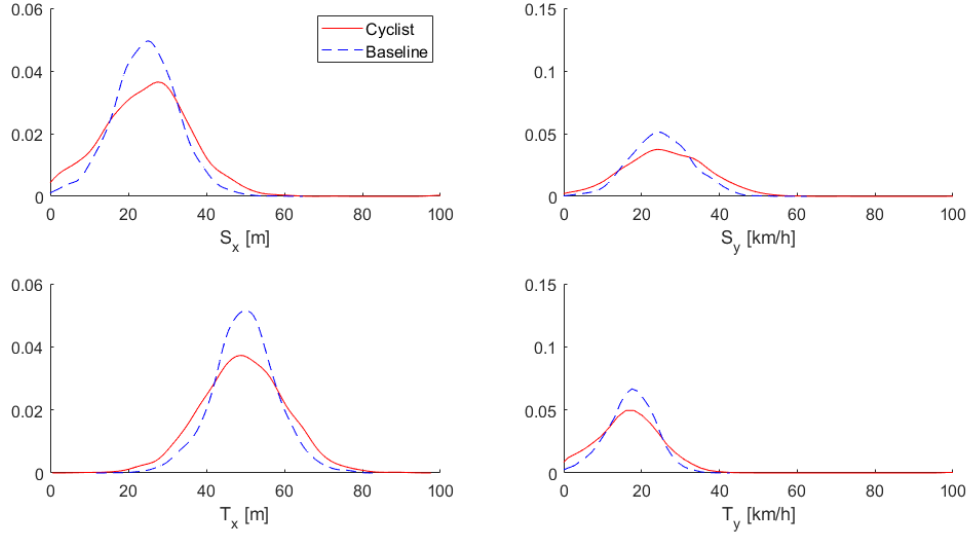
Figure 21. Prior predictive draws for S_x (travelled distance from trigger point, at start of braking), S_y (speed at start of braking), T_x (total distance travelled during braking manoeuvre) and T_y (total speed reduction during braking manoeuvre), from Schindler et al. (2021)
