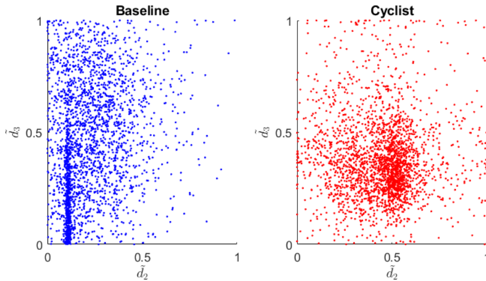
Figure 25. Posterior predictive draws of \tilde{d}_2 and \tilde{d}_3 in beta space, from Schindler et al. (2021)
