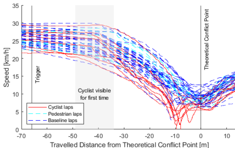
Figure 14. Speed over distance travelled by HGV drivers in the first right turn manoeuvre (cyclist encounters), adapted from Schindler and Bianchi Piccinini (2021)
