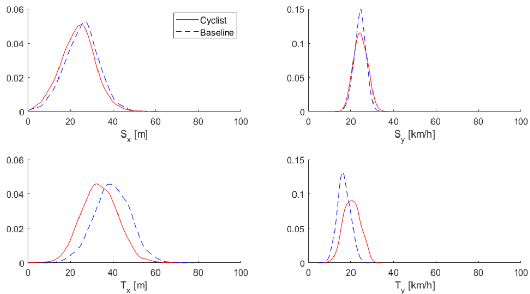
Figure 24. Posterior predictive draws for S_x (travelled distance from trigger point, at start of braking), S_y (speed at start of braking), T_x (total distance travelled during braking manoeuvre) and T_y (total speed reduction during braking manoeuvre), from Schindler et al. (2021)
