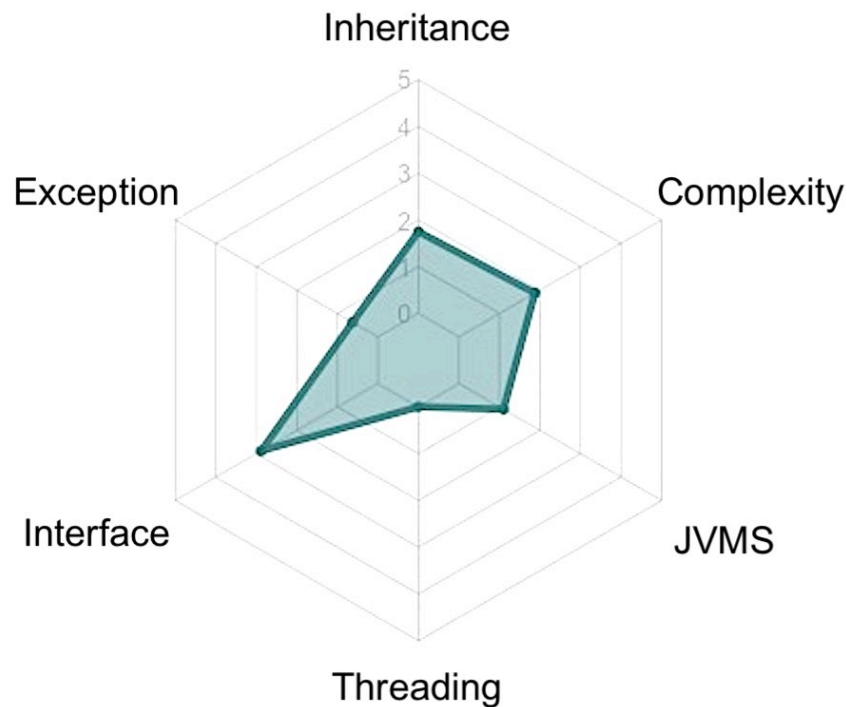
Figure 4 Example of ATDx radar-chart of the project Apache Groovy ( https://github.com/apache/groovy ), generated by considering the SonarQube AR_i^{SQ} rules utilized in the empirical evaluation. Full-size DOI: 10.7717/peerjcs.833/fig-4
