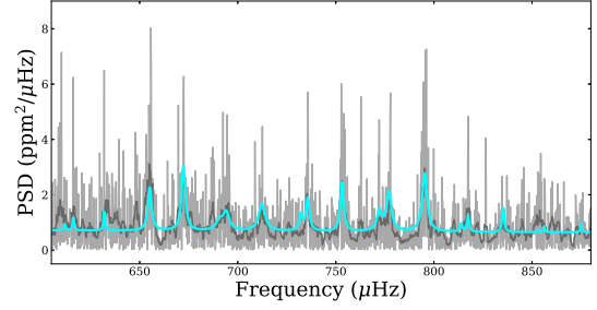
Figure 1. PSD of the asteroseismic optimized light curve (in light grey) at the natural resolution (no oversampling is performed) with a 11 points boxcar-smoothed version over-plotted in dark grey. The result of the APOLLINAIRE fit is shown in cyan.
