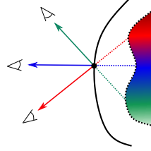
Figure 4.2: Illustration of the shape-radiance ambiguity. A single point on a false surface (solid) can satisfy the incoming radiance to the cameras through view-dependent colors, even though these rays correspond to three distinct points on the real surface (dotted).
