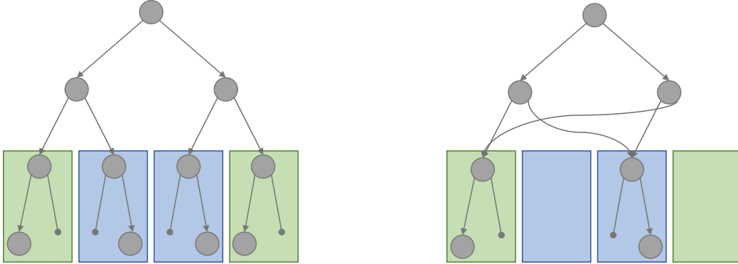
Figure 2.3: A comparison between a Sparse Voxel Octree (left) and a Sparse Voxel DAG (right) data structure. In a Sparse Voxel DAG identical subtrees are identified, and all but a unique copy of each such subtree is replaced with a pointer.
