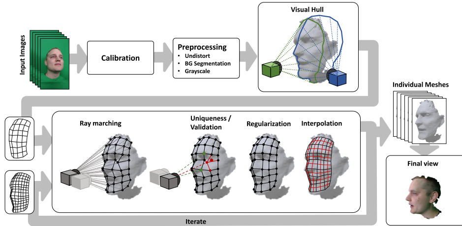
Figure 3.2: An overview of the pipeline described in Paper II . The pipeline includes multiple steps, starting with an input of one frame per camera, and ending with a final view rendered from a virtual camera. The whole pipeline is executed in \sim 14\text{ms} .
