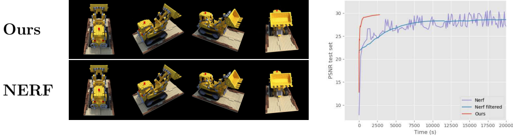
Figure 4.1: Results from our method in Paper IV compared to NERF without view-dependence. Our method produces novel views of similar quality as NERF, but in a fraction of the time as can be seen in the graph to the right.
