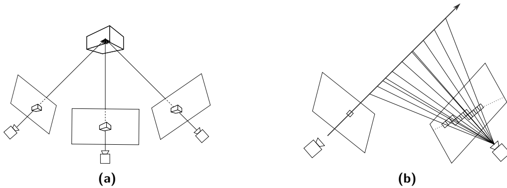
Figure 3.1: In (a), an illustration of depth reconstruction via triangulation is shown. As long as the same point of an object can be correctly identified (and is visible) in each image, and that the camera intrinsics and poses are known, it is possible to infer the position of this point in 3D. In (b), a ray is followed through a pixel of one image. This ray is projected on another image, and a matching pixel can be searched for along this line. Note that the angle between the two cameras determine the effective depth resolution of this search.
