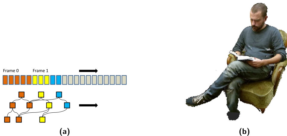
Figure 2.4: In (a) , an illustration of a temporal DAG is shown. It has a root node per frame, which are sorted in time. Each unique node is stored as early as possible in the stream, while subsequent occurrences just point back to this piece of data. In (b) , we see a frame from data captured with KinectV2 depth cameras to evaluate our algorithm in Paper I .
