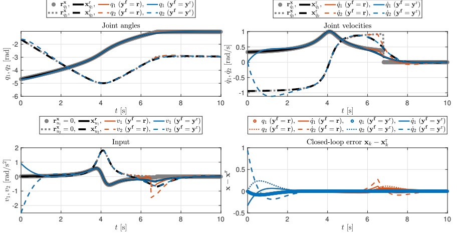
Figure 2.2: Closed-loop simulation for the initial time k = 167 and initial condition (x_1, x_2) = (-4.69, -1.62, 0, 0) . The reference trajectory \mathbf{r}(\tau) = (\mathbf{r}^x(\tau), \mathbf{r}^u(\tau)) is represented by the gray lines, while the feasible reference trajectory \mathbf{y}^r is represented by the black lines. The orange lines show the closed-loop trajectories for the practical formulation (2.4) while the blue trajectories show the closed-loop behavior of the ideal formulation (2.12).
