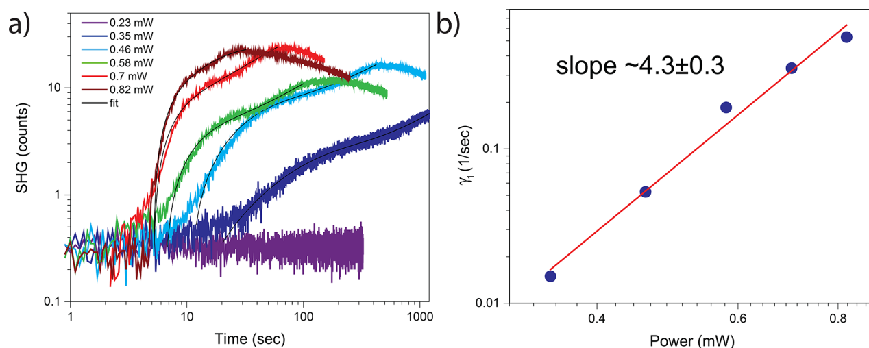
Figure 4. (a) Time evolution of the SHG signal intensity of monolayer \text{ReS}_2 with different excitation power at 1040 nm in log–log scale. The signal at each laser power was collected by parking a focused laser beam at a certain location on the flake and monitoring the \text{SHG}(t) , as the 1\text{T}' -to- 2\text{H} phase transition proceeds. Several laser intensities were used at different locations of the same monolayer flake to monitor the power dependence of the patterning process. (b) Log–log plot of the SHG growth rate vs laser power, showing the slope of 4.3 \pm 0.3 , which indicates a highly nonlinear origin of the transition. Error bars are smaller than the symbol size.
