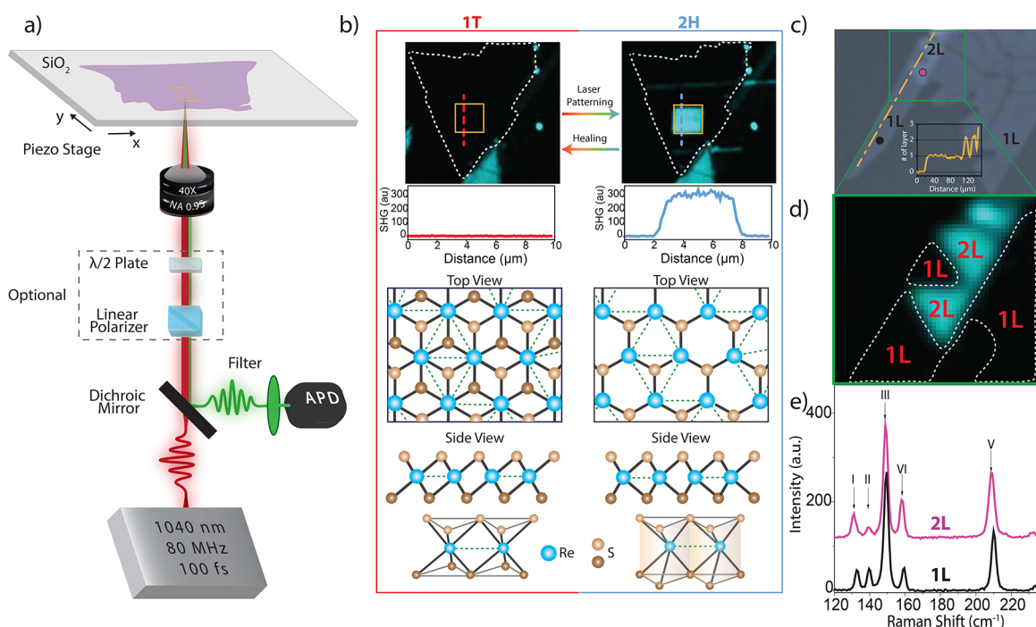
Figure 1. (a) Schematic diagram of the experimental setup for SHG measurements and laser patterning. (b) Spatial SHG map of an unpatterned monolayer \text{ReS}_2 marked with a white dotted line and an SHG intensity profile analyzed along the dashed line (left, top) and a laser-patterned monolayer (marked with an orange box) and analyzed SHG intensity profile of the patterned area (right, top). A substantial ( \sim 2 orders of magnitude) enhancement of the SHG is observed for the laser-patterned monolayer. All SHG images are presented in false color. (bottom) Crystalline structure of the 1T (left) and 2H phases (right). Green dashed lines schematically illustrate formation of Re–Re bonds in \text{ReS}_2 . (c) Optical microscope image of the mono- and bilayer \text{ReS}_2 . (inset) Gray scale contrast profile relative to the substrate along the dashed–dotted line profile. (d) SHG spatial map of the unpatterned mono- and bilayer \text{ReS}_2 on a glass substrate. Notice a considerably higher SHG signal from the bilayer region. (e) Raman spectra of \text{ReS}_2 mono- and bilayer measured at the positions marked with black and pink circles in c, respectively. A_g -like and E_g -like Raman modes are labeled as I and III, respectively.
