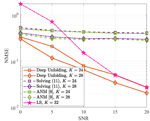
Fig. 4: Impact of training overhead on estimating the cascaded channel for a 1 \times 16 SIMO system with N = 32 and L_1 = L_2 = 1 . Deep unfolding vs. LS estimation, ANM [9], and the direct solution of (11) [15].
