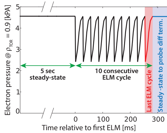
Figure 6. Evolution of the electron pressure close to the pedestal top ( \rho_{\text{TOR}} = 0.9 ) in the JETTO simulations. After 5 seconds of simulation time with steady kinetic profiles, 10 consecutive ELM cycles are simulated. In what follows, the results shown belong to the evolution of the last ELM cycle of the sequence, indicated with the red shaded area. Some simulations were continued with fixed pre-ELM profiles to test the diffusion term in eq. (4). This is indicated with the blue shaded area.
