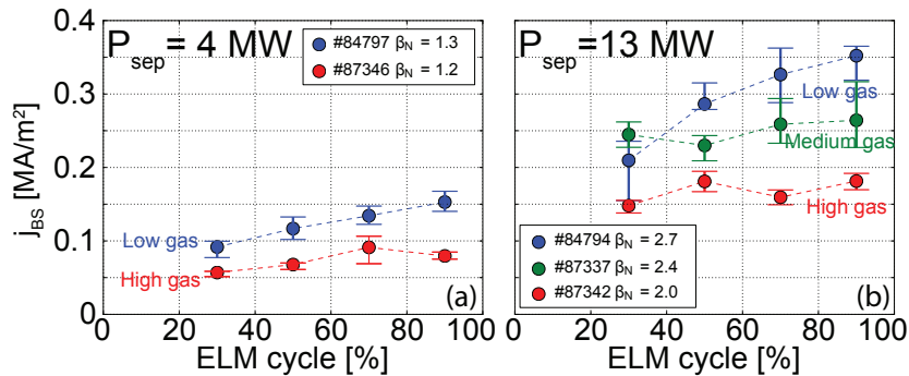
Figure 4. Evolution of peak j_{\text{BS}} during the ELM cycle in type I ELMy H-modes at low ( 2.8 \cdot 10^{21} e/s), medium ( 8.4 \cdot 10^{21} e/s) and high ( 18 \cdot 10^{21} e/s) gas rates at constant P_{\text{sep}} : (a) lowest power and (b) highest power of the power and gas scans dataset.
