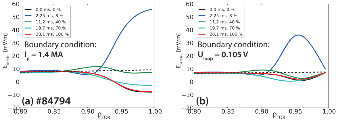
Figure 8. Inter-ELM evolution of the parallel electric field profiles for pulse #84794 ( T_{e,PED} = 0.9 keV). (a) Total current held constant as boundary condition, (b) loop voltage at the separatrix held constant as a boundary condition. The electric field significantly increases during the ELM crash (blue curve) as a response to the drop in the edge bootstrap current. The dashed lines show the time-average of the electric field profile over the ELM cycle, which is close to the fully diffused electric field.
