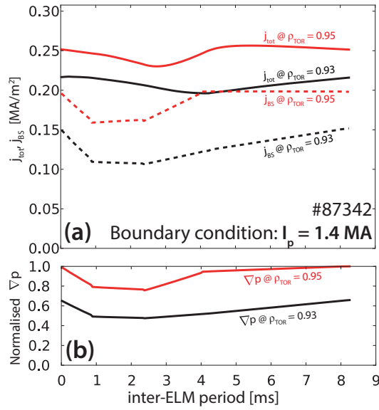
Figure 11. (a) Inter-ELM evolution of the total (solid curves) and bootstrap current (dashed curves) profiles at two radial coordinates close to the peak, \rho_{\text{TOR}} = 0.95 , and close to the pedestal top \rho_{\text{TOR}} = 0.93 in #87342 with I_p = \text{const.} boundary condition. (b) The evolution of the pressure gradient in the inter-ELM cycle.
