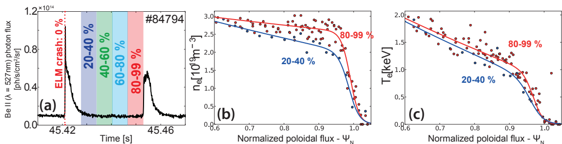
Figure 1. (a) The ELM cycle is normalised to a relative time scale (from 0 % to 100 %) and divided into 20 % long intervals. The ELM marker is the Be II ( \lambda = 527 nm) photon flux measured at the inner divertor. (b) and (c) The n_e and T_e experimental data for the 20-40 % and 80-99 % intervals in #84794.
