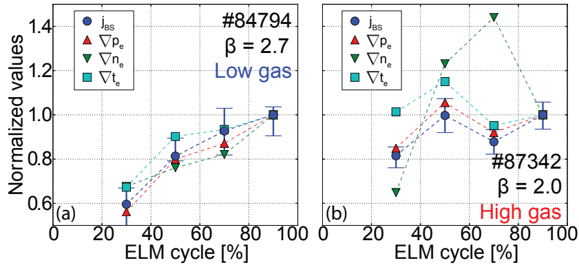
Figure 5. Inter-ELM evolution of peak j_{BS} and peak of p_e , n_e , T_e gradients at low and high gas rates at P_{sep} = 13 MW. All values are normalised to the pre-ELM phase. The error bars are shown only for peak j_{BS} to avoid overcrowding of the plot, but all data points have error bars of magnitude similar to those shown.
