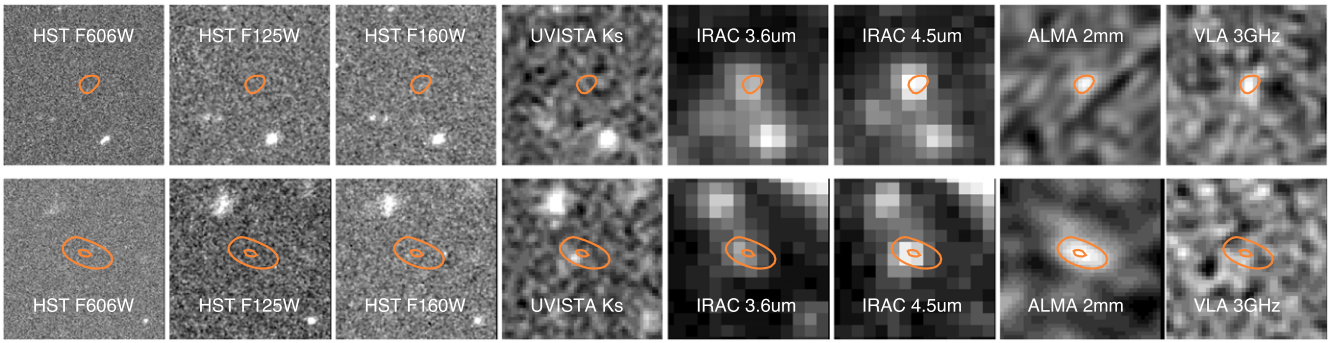
Figure 3. 8'' \times 8'' multiwavelength cutouts of MORAs-5 (top) and MORAs-9 (bottom) from HST ACS/F606W, HST WFC3/F125W, HST WFC3/F160W, UltraVISTA Ks -band, Spitzer 3.6 \mu\text{m} and 4.5 \mu\text{m} , ALMA 2 mm, and VLA-3 GHz. Orange contours in each frame show the 5\sigma contours (3 and 5\sigma for MORAs-9) from the 2 mm imaging.
