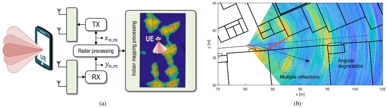
Fig. 1. (a) Considered joint communication and sensing/radar scenario in mm-wave 5G NR network, for user terminal based mapping applications. (b) Example measurement based illustration of selected indoor mapping challenges related to angular degradation as well as to multi-bounce phenomenon at 28 GHz.
