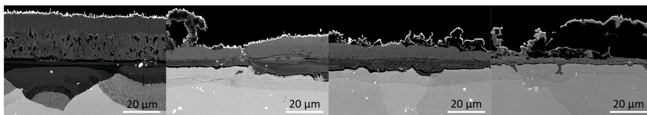
Fig. 13. SEM-BSE cross section images of a) Fe5CrAlSi, b) Fe10CrAlSi, c) Fe15CrAlSi, and d) Fe20CrAlSi after being exposed to 5% O 2 + 20% H 2 O at 600 °C with KCl present for 168 h in a tube furnace.
