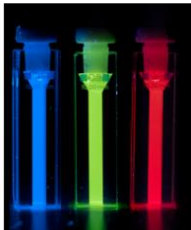
Figure 6.7. Left: structure of the ST-7-8 copolymer. m:n = 4:1 . Right: the photo of fluorophores alone (left to red: perylene, DAEg(c) and DAEr(c)) in the micelles upon 365 nm excitation.
