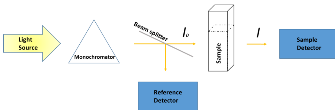
Figure 3.1. Schematic setup of a UV-vis absorption spectroscopy.
