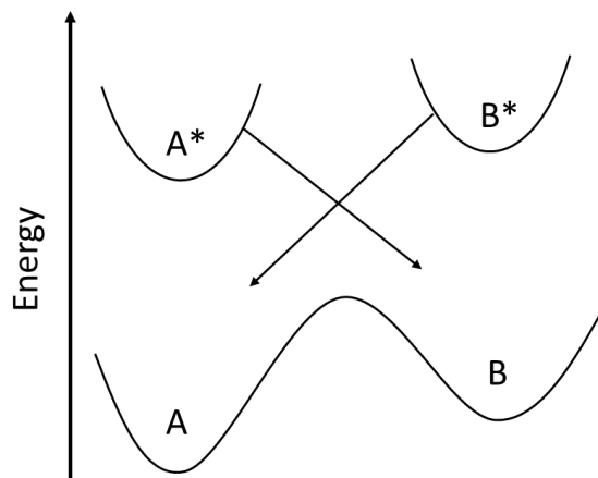
Figure 4.1. The light-induced isomerization by light (arrows) between two isomers, A and B.
