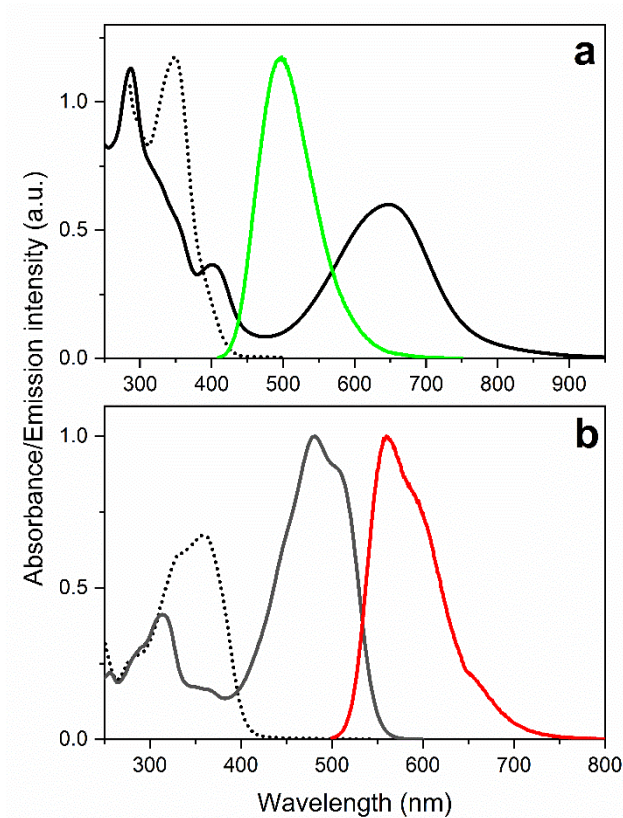
Figure 5.7. Absorption and emission spectra of Dasy (shown in a) and DAE9 (shown in b). The black dotted lines stand for the absorption spectra of the open isomers, the black solid lines stand for the absorption spectra of closed isomers. The green solid line stands for the emission of Dasy(o) and the red solid lines stand for the emission spectrum of DAE9(c).
