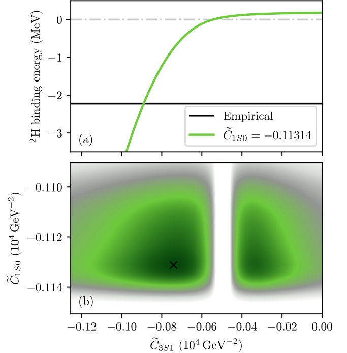
FIG. 9. (a) {}^2\text{H} binding energy as a function of \tilde{C}_{3S1} with \tilde{C}_{1S0} = -0.11314 \times 10^4 \text{ GeV}^{-2} . (b) LO posterior evaluated on a lattice. The black cross marks the MAP point indicated on the diagonal in Fig. 1, i.e., (\tilde{C}_{1S0}, \tilde{C}_{3S1}) = (-0.11312, -0.07416) \times 10^4 \text{ GeV}^{-2} .
