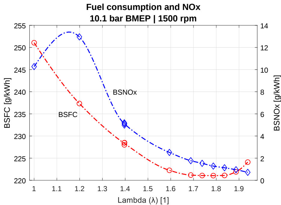
Figure 5. Engine out Brake specific \text{NO}_x emissions (BSNOx) and brake-specific fuel consumption (BSFC), versus lambda. The graph of \text{NO}_x illustrates how the \text{NO}_x -emissions increase when lambda is increased from stoichiometry to slightly lean, lambda = 1.2, and then steadily decrease when exceeding lambda = 1.4. Additionally, the graph of BSFC illustrates an increase in fuel consumption at very lean operation (lambda > 1.85) due to increased combustion instability.
