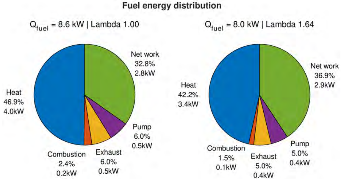
Figure 4. Indicated distribution of provided fuel energy at an engine speed of 2000 rpm and \sim 2.62 bar BMEP. Left: Stoichiometric combustion. Right: Lean combustion. Experimental data obtained from measurement campaign 4. Energy balance computed according to Clasen et al. [50].
