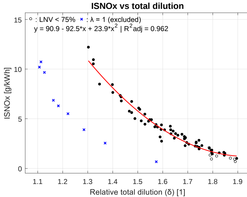
Figure 41. Correlation plot between indicated specific NO x emissions and relative total dilution. The stoichiometric points are excluded from the curve-fit due to the shift of the second derivative between lambda 1 and 1.2. Engine speed 2000 rpm, 2.62 bar BMEP engine load, CA50 = MBT.
