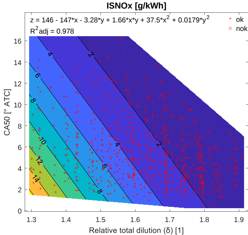
Figure 42. Regression model of ISNOx versus relative total dilution ( \delta ) and combustion phasing (CA50), at 2000 rpm and 2.62 bar BMEP of the multi-cylinder engine. *ok: combustion within stability criterions. *nok: combustion exceeding stability criterions. Stoichiometric combustion is excluded. The map and corresponding regression are derived from approximately 650 measurements.
