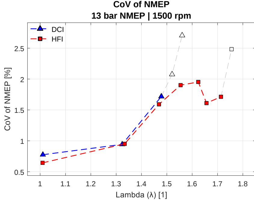
Figure 12. Example of the difference in the lean limit (air dilution tolerance) between a dual coil ignition system (DCI) and a high frequency ignition (HFI) system. As can be seen, it was possible to extend the lean limit 0.25 lambda units using the HFI system. The stability limit was set to 2% CoV of NMEP in this case. Gray lines and open markers denote operating points exceeding the stability criterion. Data acquired from campaign 2.
