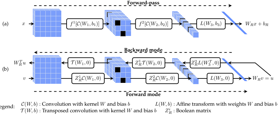
Figure 3.6: The difference between a regular forward-pass and the forward and backward modes for a two hidden layer network. (a) A regular forward-pass of x through the network. Each box showcases the operation that maps the input between the layers. The black squares indicate the neurons mapped to zero by the ReLU activation functions f^i . (b) The forward and backward modes used to estimate the slope \|W_R\|_2 . An input v is sent through the network to yield u whereupon u is sent backwards through the network. Adapted from Figure 1 in Paper IV .
