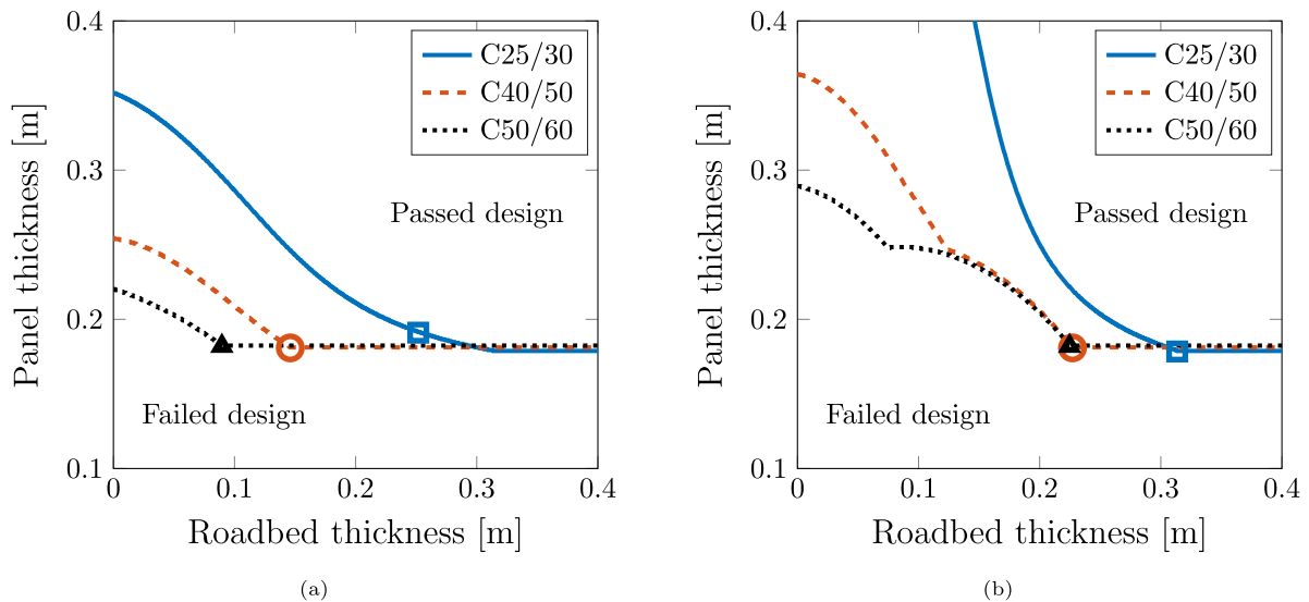
Fig. 6. Combinations of panel and roadbed thicknesses that would pass or fail the European standard 16432-2 [2] for each type of concrete when using axle load (a) 17 tonnes and (b) 25 tonnes. The markers in the figure indicate the optimised dimensions.
