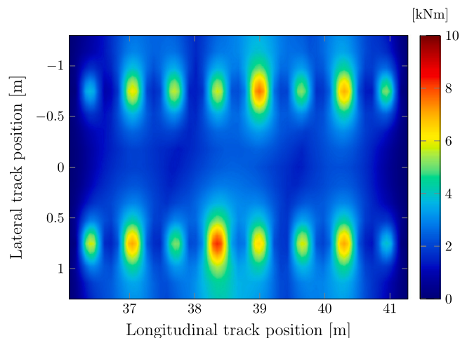
Fig. 9. Distribution of maximum bending moment that causes stress in the longitudinal direction in the concrete panel (maximum value 8.54 kNm). Vehicle speed 250 km/h, uncracked section, track class C, concrete class C25/30 and optimised dimensions from Section 5.1.
