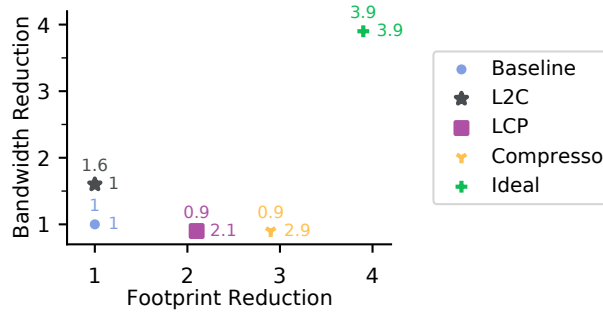
Figure 5.1: Bandwidth reduction vs. Footprint reduction for three state-of-the-art memory compression systems with identical lossless compressors. Ideal shows the achievable compression, LCP and Compresso are compacting systems, L 2 C performs no compaction.
