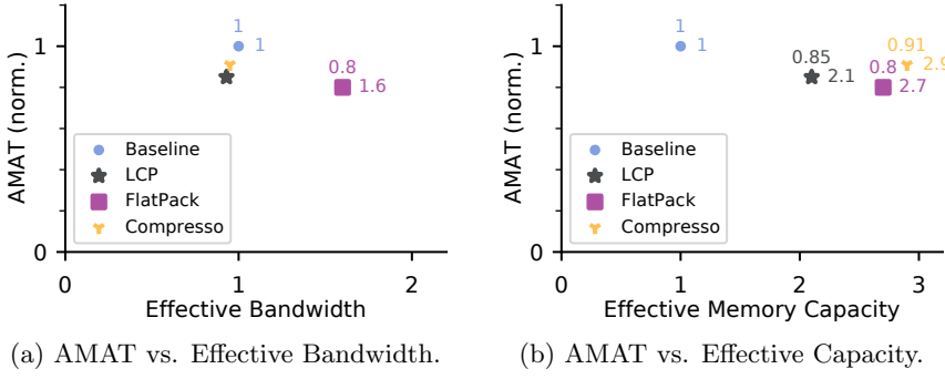
Figure 5.18: Average Memory Access Time (AMAT) weighed against the bandwidth and capacity effects of the investigated memory compaction systems.
