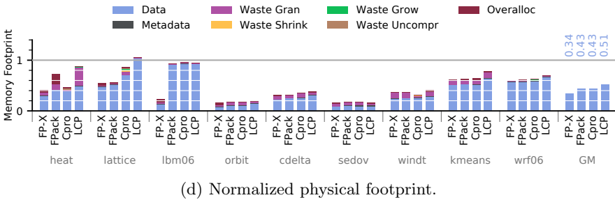
Figure 5.20: Multi-core results for FlatPack with lossy and lossless compression (FP-X), FlatPack with lossless compression (FPack), Compresso (Cpro), and LCP
