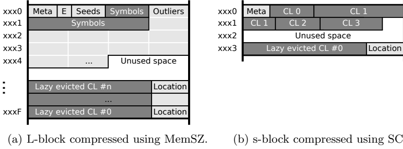
Figure 4.4: L 2 C Memory Block formats. Large blocks ( L-blocks ) are lossily compressed, Small blocks ( s-blocks ) are losslessly compressed.
