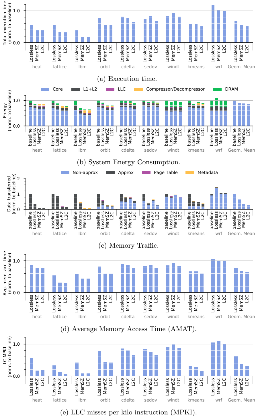
Figure 4.10: Evaluation of the L^2C memory compression design and comparison with competing designs.
