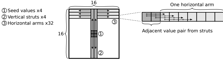
Figure 3.4: SZ Compression adapted to a 2D block
