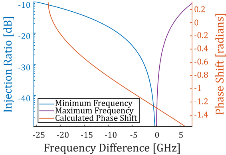
Figure 3.5: Locking conditions derived from the modified rate equations, equations 3.18 and 3.19. The minimum offset frequency for locking is in blue, and the maximum is in purple. The phase shift curve in orange varies between the inverse cotangent of the linewidth enhancement factor, \alpha , for minimum detuning and -\frac{\pi}{2} for maximum detuning. The phase shift curve given corresponds to an injection ratio of -17.5 dB (which corresponds itself to a maximum allowable detuning, \Delta\omega of approximately 28 GHz). For all simulations, \kappa is set to 25 \times 10^9 , and \alpha is set to 3.
