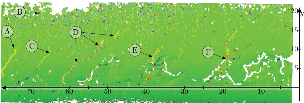
Figure 7. DIC results, viewed from above the microscopy sections. The black rectangle at x = y = 0 shows the location of the reference mark, and axes correspond to the axes in Figure 9 with dimensions in mm. The same strain scale as in Figure 4(b) is used. The coloured circles show the end-points of the cracks marked with the corresponding translucent colour in Figure 9
