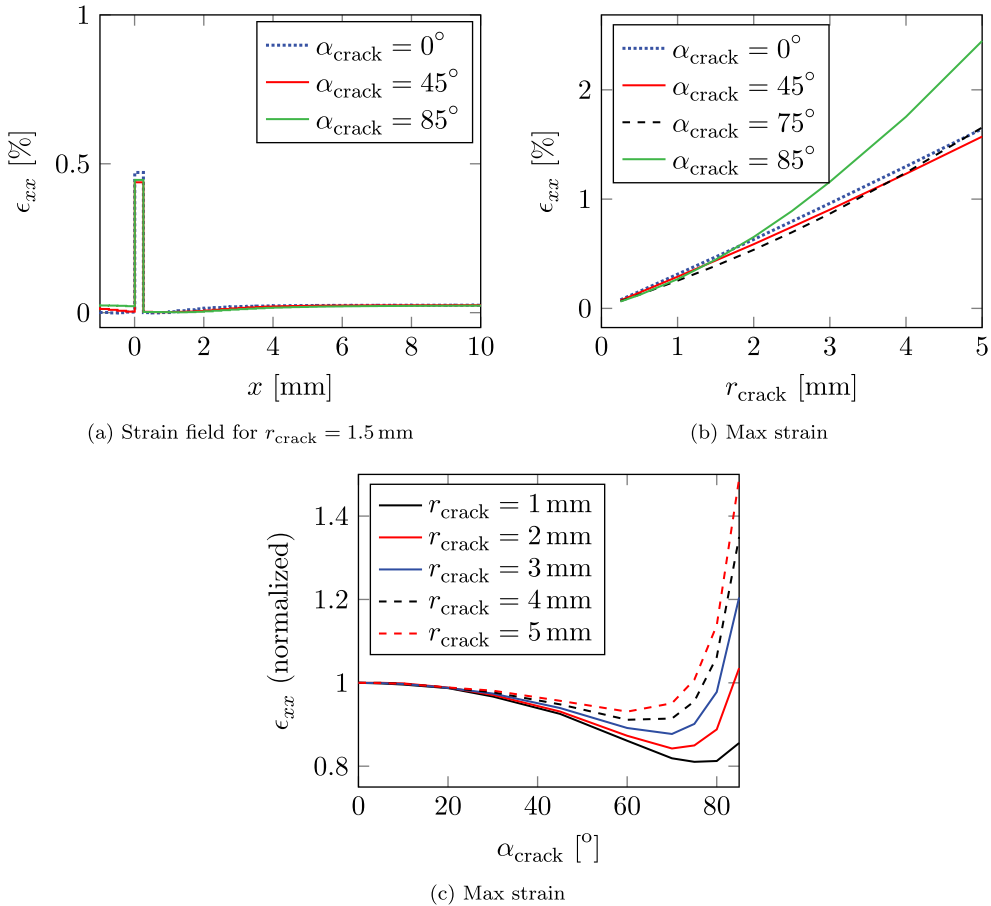
Figure 14. FE-modelling results.
