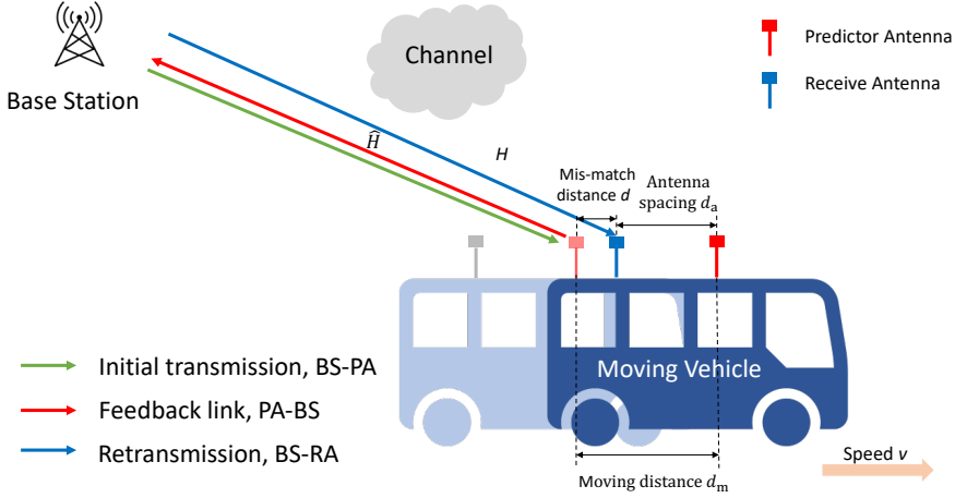
Figure 3.1: The PA concept with HARQ.
