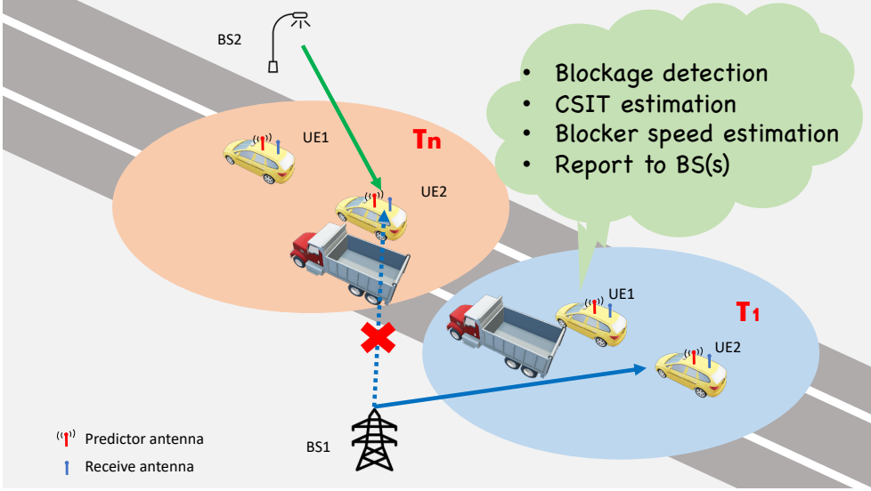
Figure 4.2: Illustration of the proposed large-scale cooperative PA (LSCPA) setup from Paper F [122].
