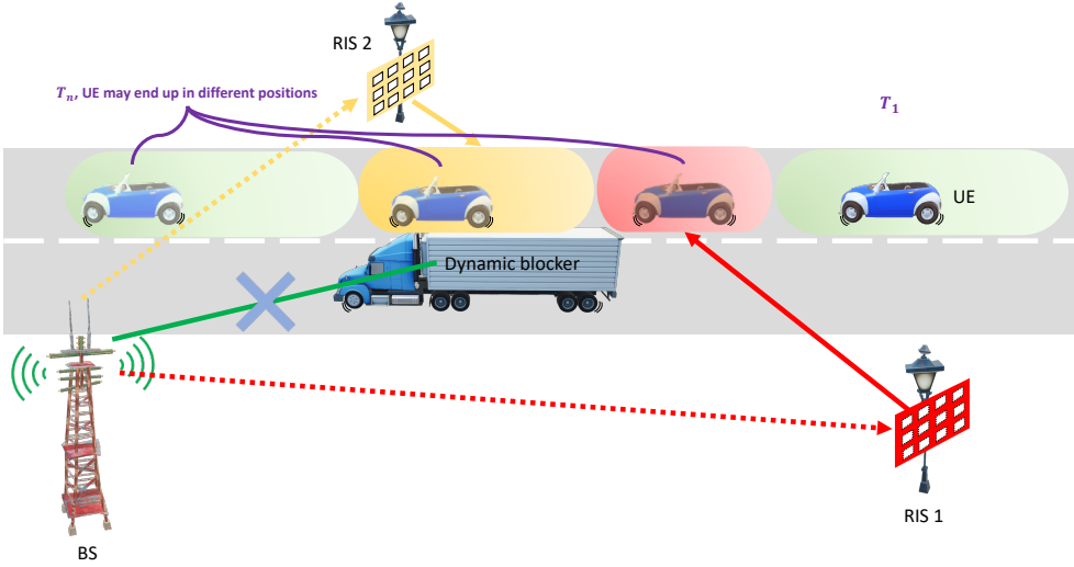
Figure 4.3: Illustration of the proposed LSRPA setup [Paper G].
