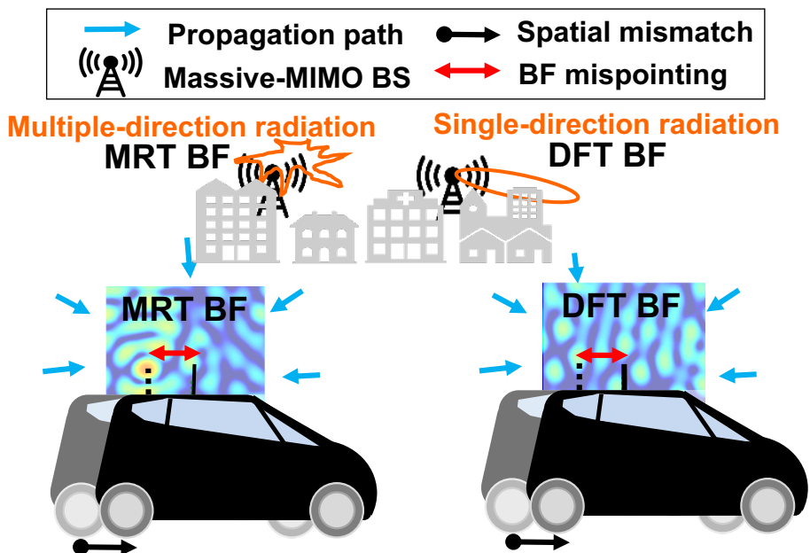
Figure 4.1: Illustration of massive MIMO schemes in PA systems with spatial mismatch [117] (the appended Paper E).
