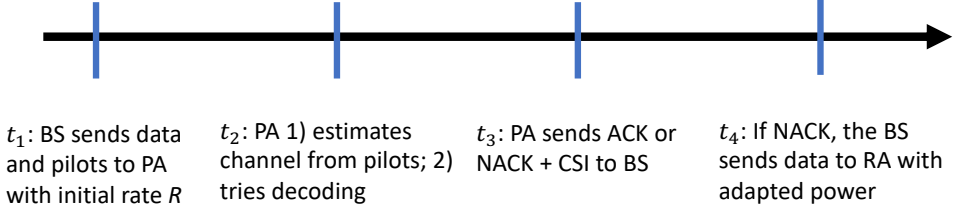
Figure 3.2: Time structure for the proposed outage-constrained power allocation in the HARQ-based PA system from Paper C [115].
