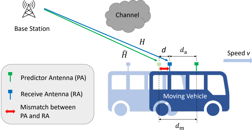
Figure 1.1: The PA concept with spatial mismatch problem.
