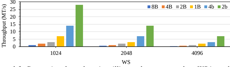
Figure 1.3: Processing throughput in million tuples per second vs. WS in tuples for an FPGA-based Single-SWAG dataflow engine [15] at 156.25 MHz with varying tuple’s value sizes from 8 bytes to 2 bits and WA = 1 tuple, showing the potential for data-compression.
