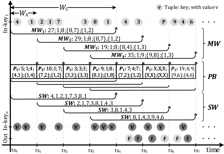
Figure 3.1: Example of time-based SWAG over a stream of tuples composed by schema, \langle ts, key, value \rangle , for parameters F = \{sum, min, max, top-2, bottom-2\} , WS = 4 time-units, WA = 1 time-unit, and K = key and internal states/values maintained by the different implementation strategies at time instance indicated by * for In-key 1 .
