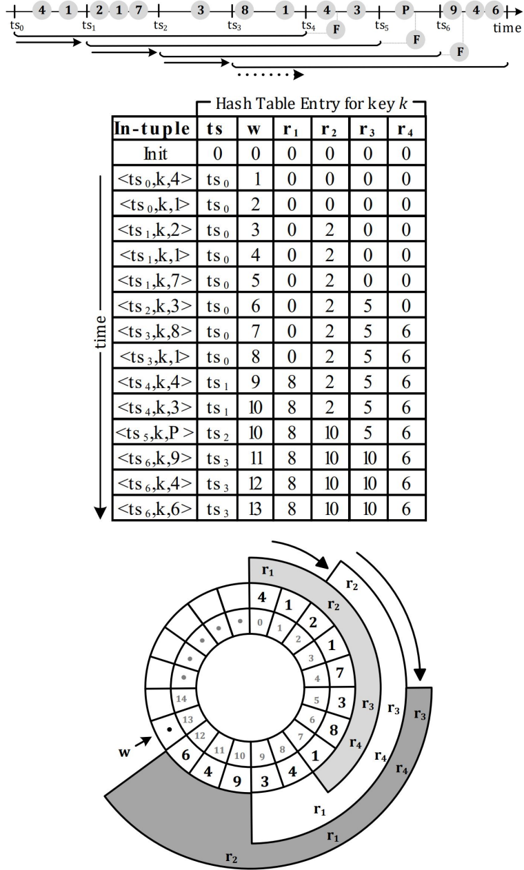
Figure 3.3: Circular buffer management. Insertion, query, and bulk eviction supported by the proposed buffer located in DRAM, which stores a single window for key k . The fields of the hash table entry for k are populated as incoming tuples arrive over time. The grey numbers in the inner circle indicate buffer indices. F-tuple indicates the output aggregate.
