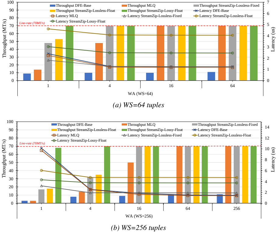
Figure 5.15: Throughput in million tuples per second (MT/s) and latency in microseconds of the various designs for WS of (a) 64 and (b) 256 tuples.
