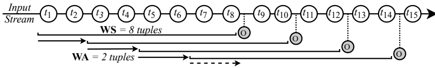
Figure 1.1: Sliding-window stream aggregation with Window Size (WS) = 8 tuples and Window Advance (WA) = 2 tuples for an input data stream, e.g. a vehicular sensor emitting tuples t_1, t_2, \dots with each tuple containing a timestamp, vehicle-ID and speed. For simplicity, only tuples from a single vehicle (key) are shown. The grey tuples indicate the aggregate output generated when the sliding-window gets full. (e.g. top-3, average, and median speed).
