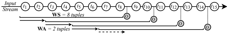
Figure 5.1: Sliding-window stream aggregation with Window Size ( WS ) = 8 tuples and Window Advance ( WA ) = 2 tuples for a input data stream, e.g. a vehicular sensor emitting tuples t_1, t_2, \dots with each tuple containing a timestamp, vehicle-ID and speed. For simplicity, only tuples from a single vehicle (key) is shown. The grey tuples indicate the aggregate output generated when the sliding-window gets full. (e.g. top-3, average, and median speed).
