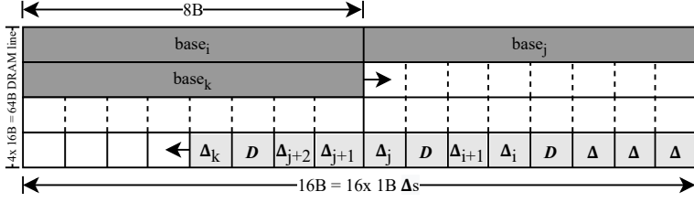
(a) Base-Delta block format of a StreamZip compressed sliding window
