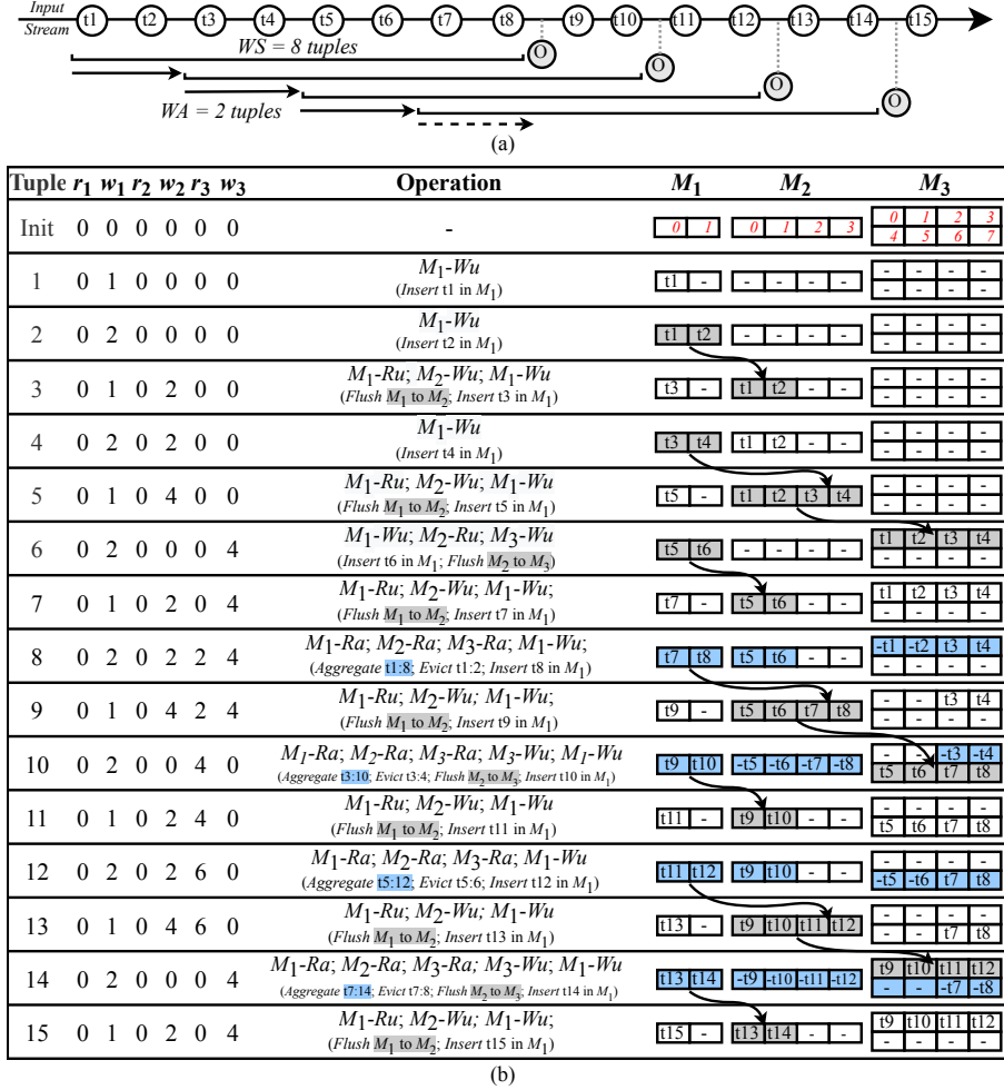
Figure 4.4: (a) A stream of tuples t1, t2, \dots , of a key aggregated with WS=8 and WA=2 tuples. (b) Hash Table metadata logic and dataflow through the memory hierarchy for the above stream. Memories configured with: v_1=2 ; v_2=4 ; v_3=8 . M_i -Wu, M_i -Ru, and M_i -Ra denotes write operation due to window update, read operation due to window update, and read operation due to aggregation in memory level i , respectively. The red numbers in the Init row indicate the indices of each memory cell. The grey and blue boxes indicate window updates and aggregation reads, respectively.
