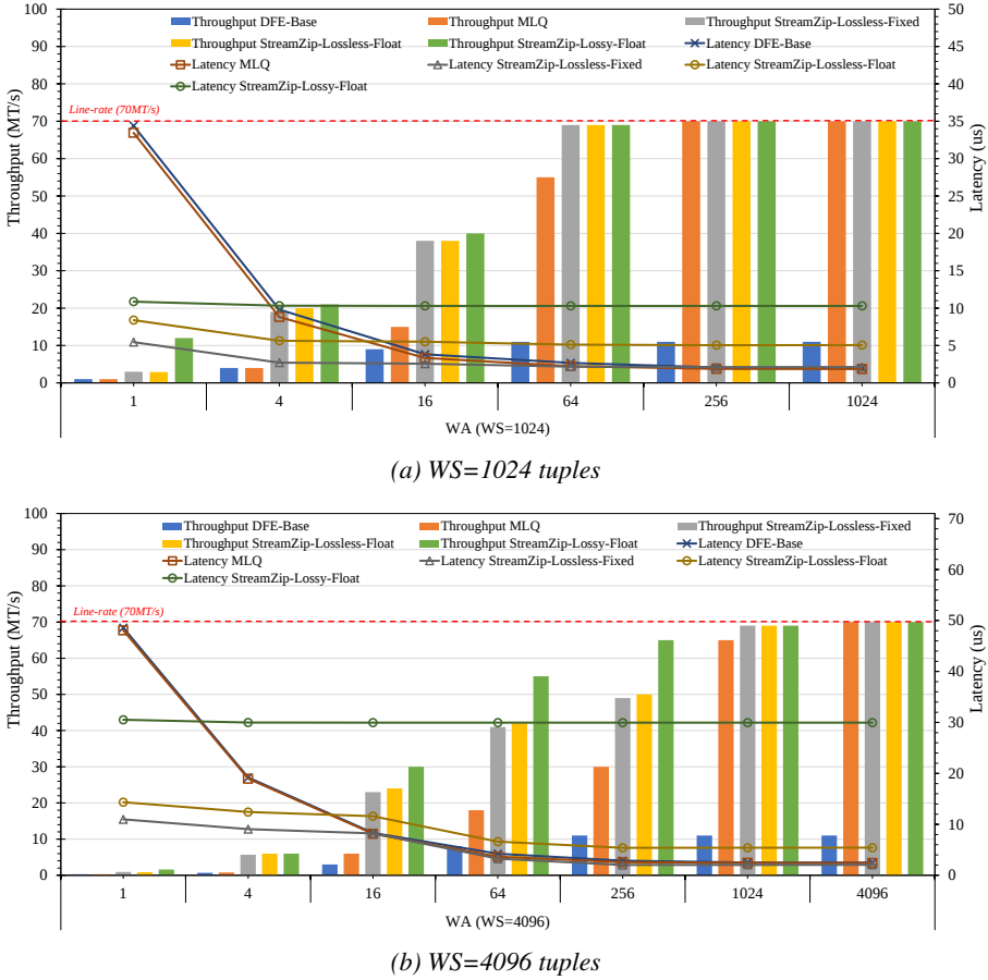
Figure 5.16: Throughput in million tuples per second (MT/s) and latency in microseconds of the various designs for WS of (a) 1k and (b) 4k tuples.
