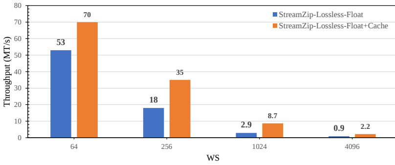
Figure 5.18: Throughput of StreamZip-Lossless-Float with Caching. A synthetic benchmark is used with a single key triggering aggregation in every cycle with WA=1 tuple.
