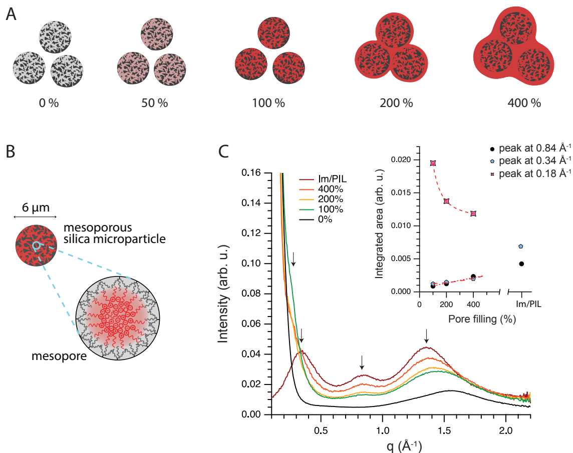
Figure 4.1: A: Illustration of, from left to right, the bare mesoporous silica microparticles ( 5\text{-C8-SiO}_2 ) and the same particles filled by an increasing amount of the Im/PIL mixture. B: Illustration of the speculated local structure inside the mesopores. C: Small-angle X-ray scattering intensity collected for the bare silica particles (black trace), different samples with varying pore filling (orange, yellow and green) and the neat Im/PIL mixture (dark red). The inset plot shows the integrated areas under selected fit peaks as a function of composition.
