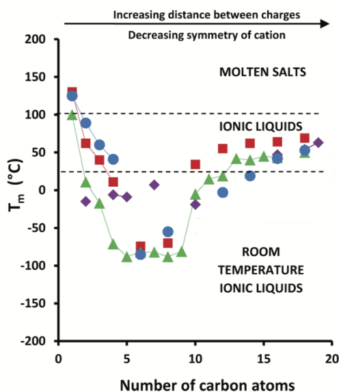
Figure 2.3: Melting temperature ( T_m ) of \text{C}_n\text{mim}^+ -based ionic liquids with different chain length and anions: hexafluorophosphate ( \text{PF}_6^- , red square), tetrafluoroborate ( \text{BF}_4^- , green triangle), bis(trifluoromethanesulfonyl)imide ( \text{TFSI}^- , purple diamond), and chloride ( \text{Cl}^- , blue circle). The figure is reproduced from reference [14] with permission from the American Chemical Society.
