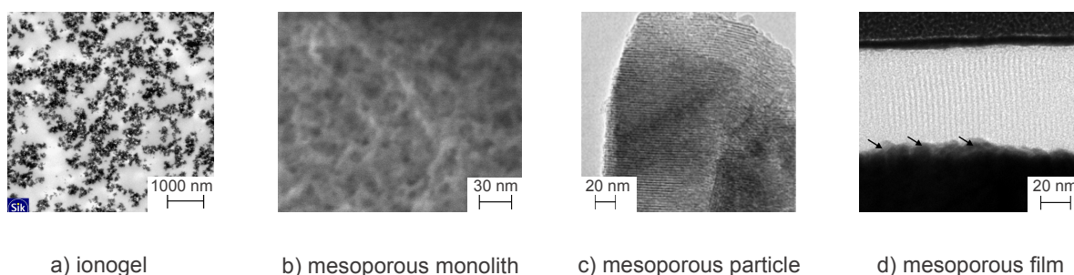
Figure 2.9: IL-templated mesoporous silicas. a) SEM of a C_6mimTFSI -based ionogel. The image is reproduced from reference [64] with permission from The Royal Society of Chemistry. b) SEM image of a C_4mimBF_4 -templated mesoporous monolith synthesised according to reference [62]. c) TEM image of a C_{16}mimBr -templated mesoporous silica particle. The image is reproduced from reference [65] with permission from Springer. d) A C_{16}mimCl -templated mesoporous silica thin film [31]
