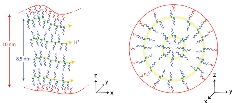
Figure 2.7: Schematic picture of the nanostructuration in the \text{HC}_8\text{imTFSI} /imidazole mixture when confined in the nanopores of hydrophobic silica (achieved by covalent bonding of trioctylsilyl-groups onto the pore wall), showing the molecular organisation along the pores (left) and across a pore section (right). The figure is reproduced from reference [5] with permission from The Royal Society of Chemistry.
