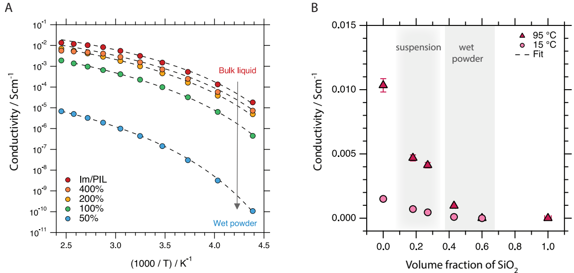
Figure 4.3: A: Arrhenius plot of conductivity values measured for samples of various pore filling covering the temperature range from -50 to 145^\circ\text{C} . Dashed lines are simple guides to the eye. B: Absolute values of conductivity measured at 15 and 95^\circ\text{C} as a function of the volume fraction of silica.
