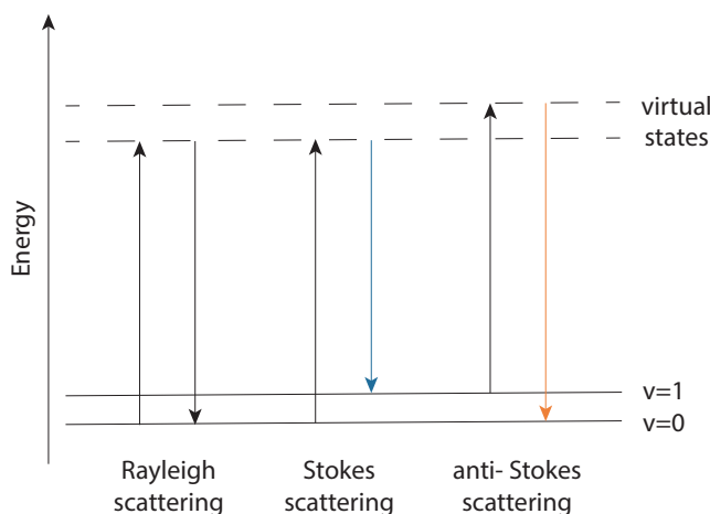
Figure 3.5: Elastic (Rayleigh) and inelastic scattering (Stokes and anti-Stokes) of an incoming photon with suitable wavelength for vibrational excitation presented on a Jablonski diagram.
