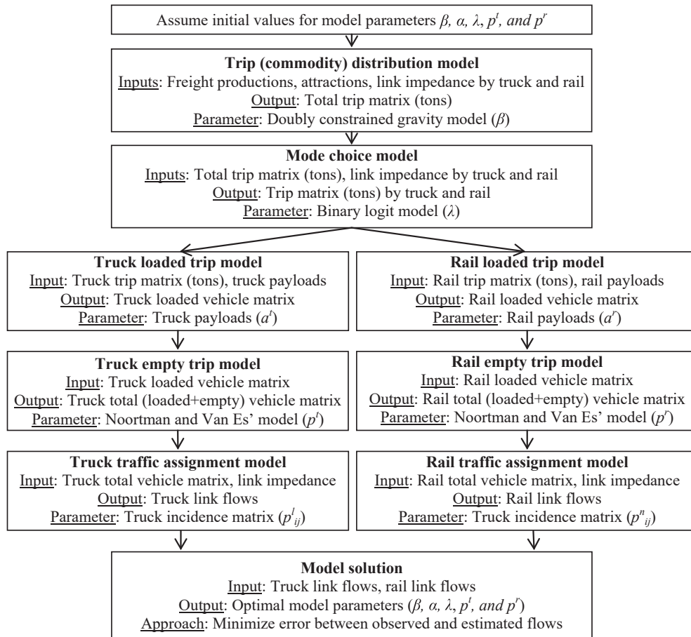
Fig. 1. FODS-MC Model Overview.
