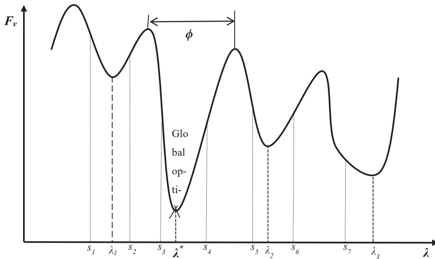
Fig. 3. Multi-Start Method.
