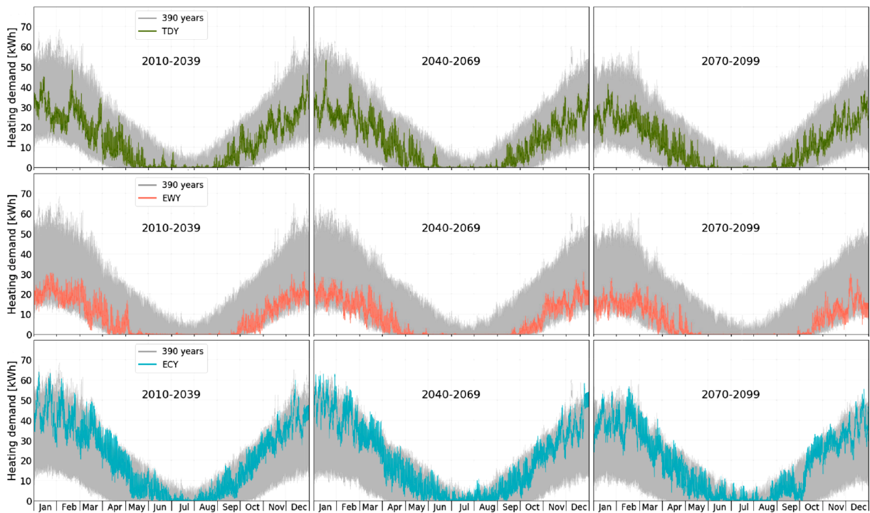
Fig. 18. Hourly profile of heating demand for 390 years (13 climate scenarios) of simulations and TDY (top), EWY (middle), and ECY (bottom).
