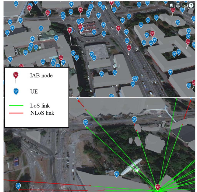
FIGURE 10. An example of the distribution of the IAB network in 3D space with OpenStreetMap.
