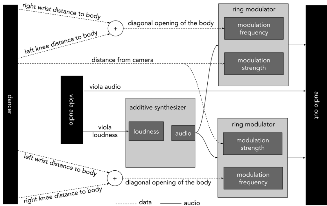
Figure 4. Additive synthesiser – Scenario 1.
