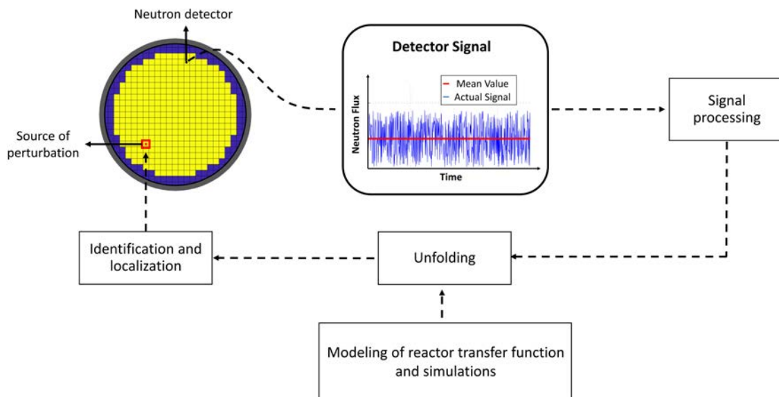
Figure 1.2 Illustration of using reactor neutron noise for core monitoring and diagnostics
