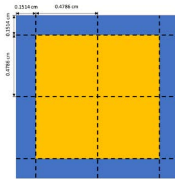
Figure 5.3 Discretization of the fuel, guide tube, or fission chamber; fine mesh for the transport sweeps
