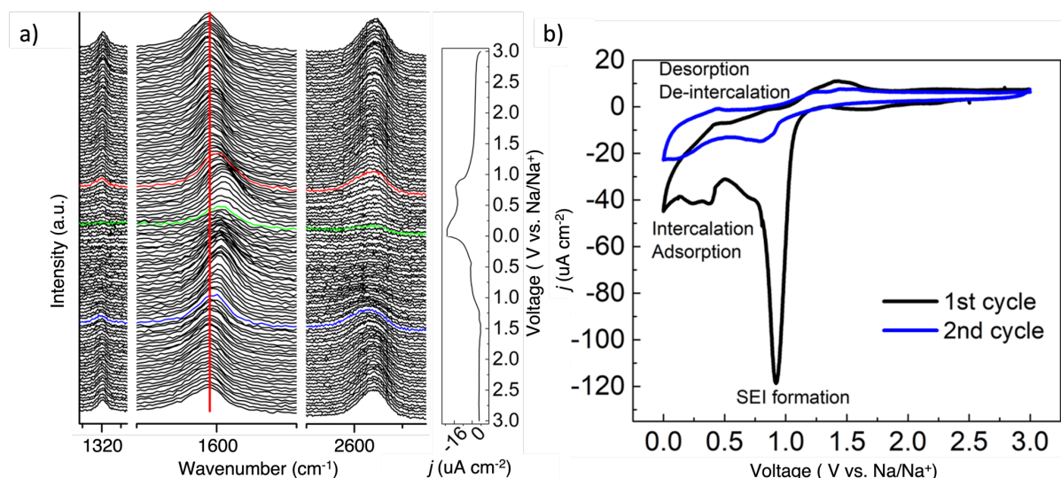
Figure 33 a) Operando Raman spectra acquired during a complete intercalation/deintercalation cycle of Na + in AB graphene; the red spectrum was measured at ca. 0.6 V, green spectrum at 0.05, and blue spectrum at ca. 1.5 V. The solid red line marks the position of the G-band b) CV curves measured during the first two cycles of Na + intercalation in AB graphene with a scan rate of 0.042 mV/s. Figure 5 from Paper I reproduced under Creative Commons Licence.
