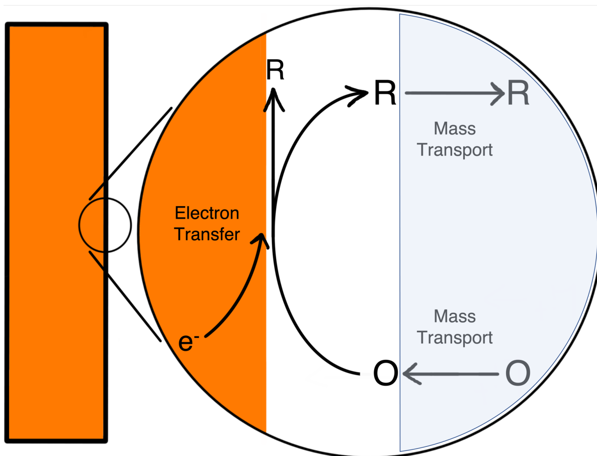
Figure 2 Schematic of the process of mass transport and electron transfer at the electrode surface.
