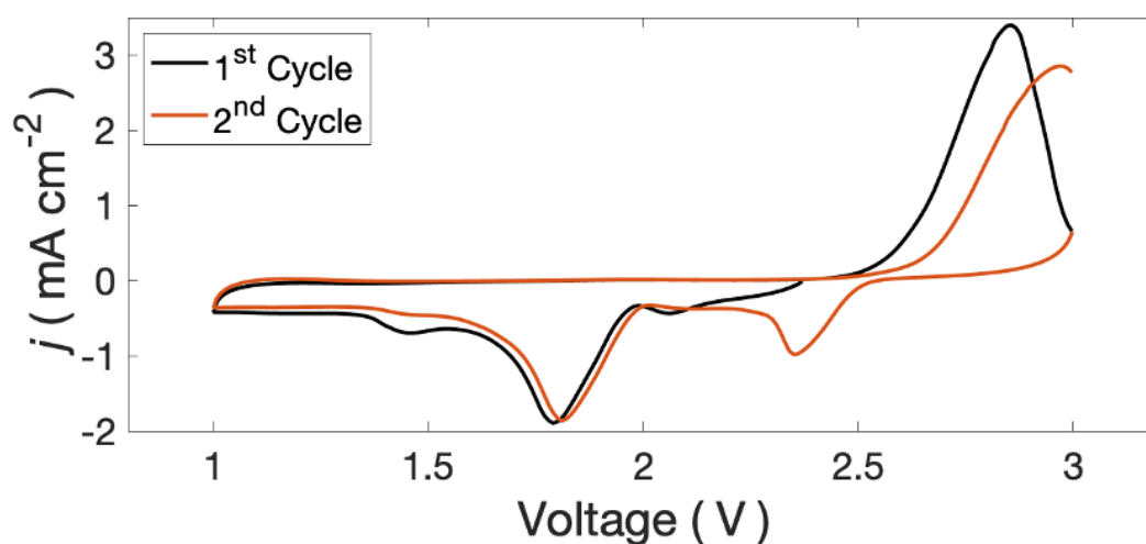
Figure 20 Example of a cyclic voltammogram for a catholyte Li-S system, showing the reduction peaks representing the conversion of \text{S}_8 to \text{Li}_2\text{S}_n ( \sim 2.4\text{V} ) and subsequent conversion to short \text{Li}_2\text{S}_n chains ( \sim 1.8\text{V} ).
