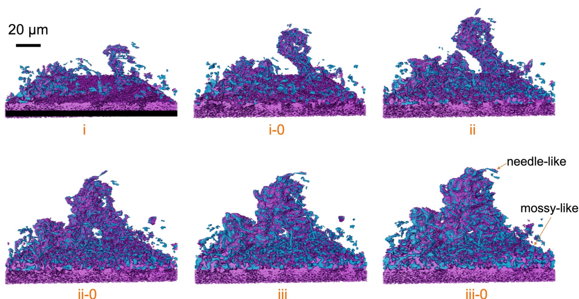
Figure 44 Evolution of Li microstructure formed by the integration of different Li dendrites. The renderings are extracted from tomograms taken during the plating at 1.0 \text{ mA cm}^{-1} for 10 min (i), 20 min (i-0), 30 min (ii), 40 min (ii-0), 50 min (iii), 1 hour (iii-0). The deposited Li is shown in blue and the phases with heavier elements are shown in purple, including the Cu substrate.
